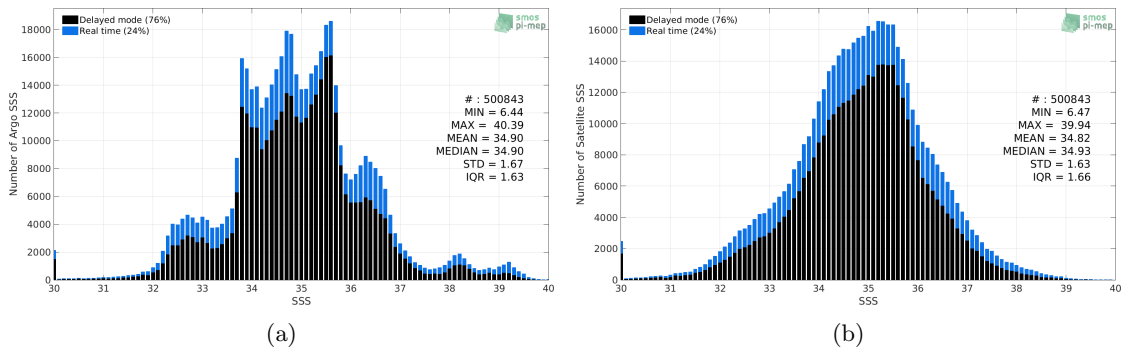
Figure 2: Histograms of SSS from Argo (a) and SMOS SSS L3 v335 - 10 Days - 25 km (CATDS-CPDC) (b) considering all match-up pairs per bins of 0.1 over the SMOS coastal zone (<800km) 60N-60S Pi-MEP region and for the full satellite product period.
