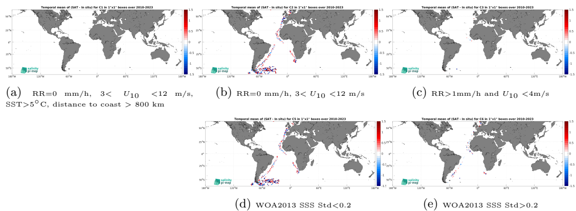
Figure 14: Temporal mean gridded over spatial boxes of size 1^\circ \times 1^\circ of \Delta\text{SSS} (SMOS SSS L2Q v333 - 0.25 Deg (CATDS-CPDC) - TSG (Polarstern)) for 5 different subdatasets corresponding to: RR=0 mm/h, 3 < U_{10} < 12 m/s, SST > 5°C, distance to coast > 800 km (a), RR=0 mm/h, 3 < U_{10} < 12 m/s (b), RR > 1mm/h and U_{10} < 4 m/s (c), WOA2013 SSS Std < 0.2 (d), WOA2013 SSS Std > 0.2 (e).
