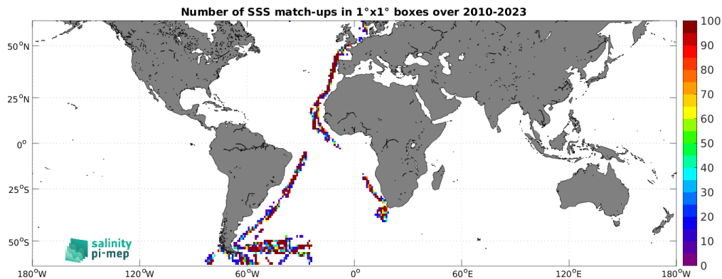
Figure 5: Number of SSS match-ups between TSG (Polarstern) SSS and the SMOS SSS L2Q v333 - 0.25 Deg (CATDS-CPDC) SSS product for the SMOS coastal zone (<800km) 60N-60S Pi-MEP region over 1^\circ \times 1^\circ boxes and for the full satellite product period.
