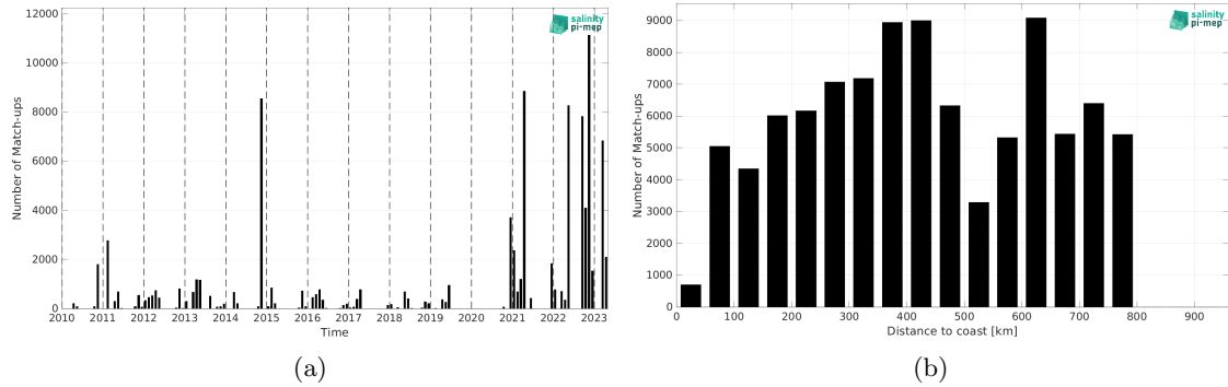
Figure 2: Number of match-ups between TSG (Polarstern) and SMOS SSS L2Q v333 - 0.25 Deg (CATDS-CPDC) SSS as a function of time (a) and as function of the distance to coast (b) over the SMOS coastal zone (<800km) 60N-60S Pi-MEP region and for the full satellite product period.
