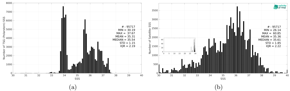
Figure 3: Histograms of SSS from TSG (Polarstern) (a) and SMOS SSS L2Q v333 - 0.25 Deg (CATDS-CPDC) (b) considering all match-up pairs per bins of 0.1 over the SMOS coastal zone (<800km) 60N-60S Pi-MEP region and for the full satellite product period.
