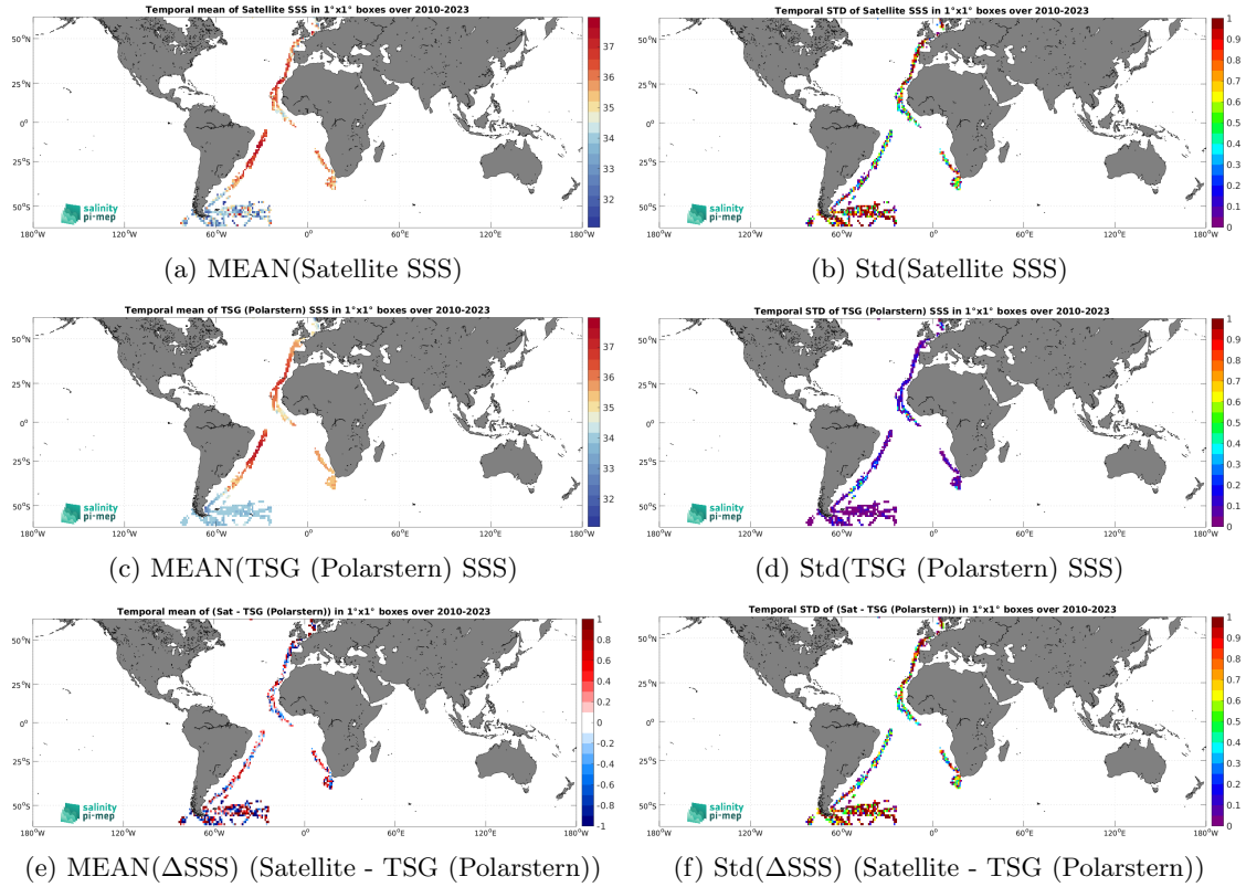
Figure 7: Temporal mean (left) and Std (right) of SSS from SMOS SSS L2Q v333 - 0.25 Deg (CATDS-CPDC) (top), TSG (Polarstern) (middle), and of \Delta SSS (Satellite - TSG (Polarstern)). Only match-up pairs are used to generate these maps.
