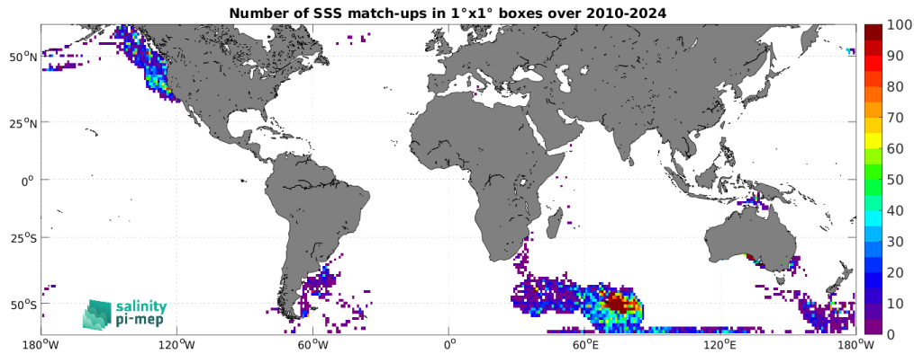
Figure 5: Number of SSS match-ups between Marine mammals SSS and the SMOS SSS L2Q v333 - 0.25 Deg (CATDS-CPDC) SSS product for the SMOS coastal zone (<800km) 60N-60S Pi-MEP region over 1°×1° boxes and for the full satellite product period.
