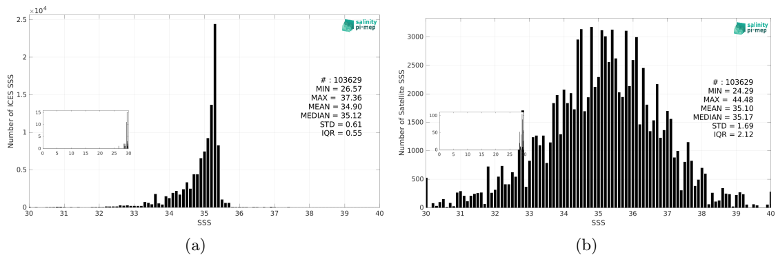
Figure 3: Histograms of SSS from ICES (a) and SMOS SSS L2Q v333 - 0.25 Deg (CATDS-CPDC) (b) considering all match-up pairs per bins of 0.1 over the SMOS coastal zone (<800km) 60N-60S Pi-MEP region and for the full satellite product period.
