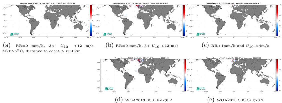
Figure 14: Temporal mean gridded over spatial boxes of size 1^\circ \times 1^\circ of \Delta SSS (SMOS SSS L2Q v333 - 0.25 Deg (CATDS-CPDC) - ICES) for 5 different subdatasets corresponding to:RR=0 mm/h, 3 < U_{10} < 12 m/s, SST >5^\circ\text{C} , distance to coast > 800 km (a), RR=0 mm/h, 3 < U_{10} < 12 m/s (b), RR >1 mm/h and U_{10} < 4 m/s (c), WOA2013 SSS Std <0.2 (d), WOA2013 SSS Std >0.2 (e).
