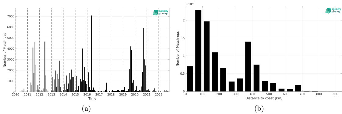
Figure 2: Number of match-ups between ICES and SMOS SSS L2Q v333 - 0.25 Deg (CATDS-CPDC) SSS as a function of time (a) and as function of the distance to coast (b) over the SMOS coastal zone (<800km) 60N-60S Pi-MEP region and for the full satellite product period.
