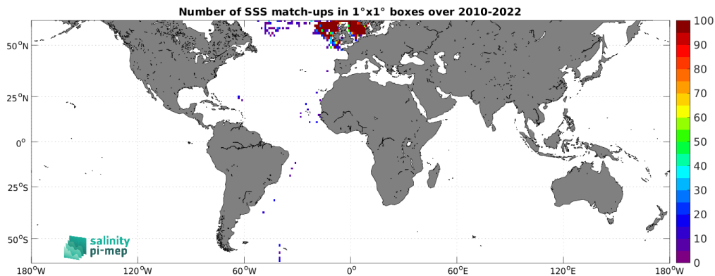
Figure 5: Number of SSS match-ups between ICES SSS and the SMOS SSS L2Q v333 - 0.25 Deg (CATDS-CPDC) SSS product for the SMOS coastal zone (<800km) 60N-60S Pi-MEP region over 1^\circ \times 1^\circ boxes and for the full satellite product period.
