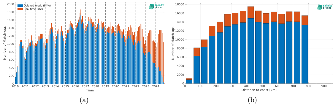
Figure 2: Number of match-ups between Argo and SMOS SSS L2Q v333 - 0.25 Deg (CATDS-CPDC) SSS as a function of time (a) and as function of the distance to coast (b) over the SMOS coastal zone (<800km) 60N-60S Pi-MEP region and for the full satellite product period.
