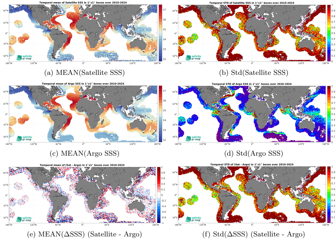
Figure 7: Temporal mean (left) and Std (right) of SSS from SMOS SSS L2Q v333 - 0.25 Deg (CATDS-CPDC) (top), Argo (middle), and of \Delta SSS (Satellite - Argo). Only match-up pairs are used to generate these maps.
