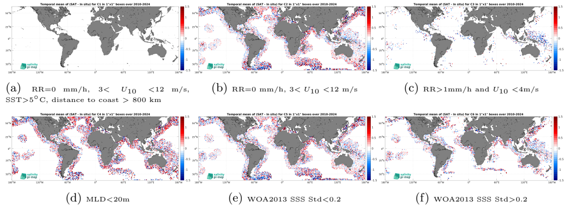
Figure 14: Temporal mean gridded over spatial boxes of size 1^\circ \times 1^\circ of \Delta\text{SSS} (SMOS SSS L2Q v333 - 0.25 Deg (CATDS-CPDC) - Argo) for 6 different subdatasets corresponding to:RR=0 mm/h, 3 < U_{10} < 12 m/s, SST>5°C, distance to coast > 800 km (a), RR=0 mm/h, 3 < U_{10} < 12 m/s (b), RR>1mm/h and U_{10} < 4 m/s (c),MLD<20m (d),WOA2013 SSS Std<0.2 (e),WOA2013 SSS Std>0.2 (f).
