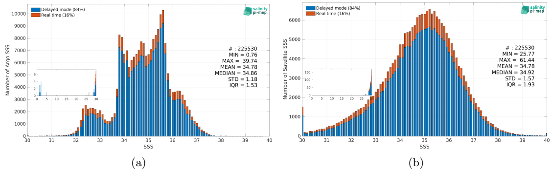
Figure 3: Histograms of SSS from Argo (a) and SMOS SSS L2Q v333 - 0.25 Deg (CATDS-CPDC) (b) considering all match-up pairs per bins of 0.1 over the SMOS coastal zone (<800km) 60N-60S Pi-MEP region and for the full satellite product period.
