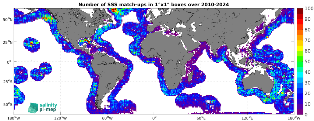
Figure 5: Number of SSS match-ups between Argo SSS and the SMOS SSS L2Q v333 - 0.25 Deg (CATDS-CPDC) SSS product for the SMOS coastal zone (<800km) 60N-60S Pi-MEP region over 1^\circ \times 1^\circ boxes and for the full satellite product period.
