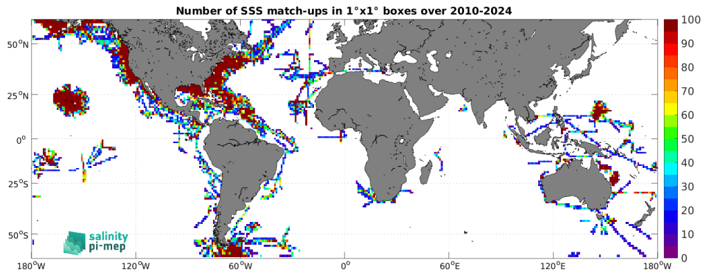
Figure 5: Number of SSS match-ups between TSG (SAMOS) SSS and the SMOS SSS L3 v332 - 9 Days (CATDS-CPDC) SSS product for the SMOS coastal zone (<800km) 60N-60S Pi-MEP region over 1^\circ \times 1^\circ boxes and for the full satellite product period.
