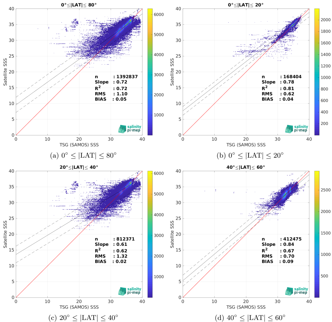
Figure 10: Contour maps of the concentration of SMOS SSS L3 v332 - 9 Days (CATDS-CPDC) SSS (y-axis) versus TSG (SAMOS) SSS (x-axis) at match-up pairs for different latitude bands. For each plot, the red line shows x=y . The black thin and dashed lines indicate a linear fit through the data cloud and the \pm 95\% confidence levels, respectively. The number match-up pairs n , the slope and R^2 coefficient of the linear fit, the root mean square (RMS) and the mean bias between satellite and in situ data are indicated for each latitude band in each plots.
