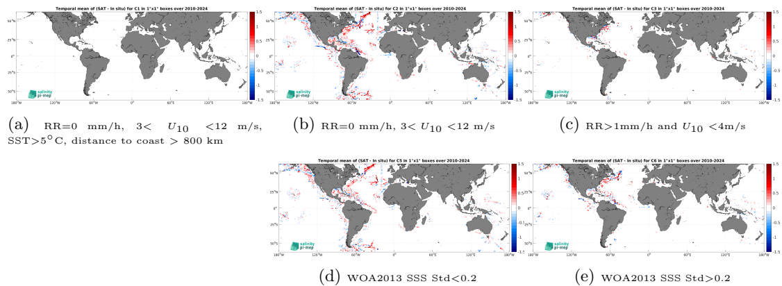
Figure 14: Temporal mean gridded over spatial boxes of size 1^\circ \times 1^\circ of \Delta SSS (SMOS SSS L3 v332 - 9 Days (CATDS-CPDC) - TSG (SAMOS)) for 5 different subdatasets corresponding to:RR=0 mm/h, 3 < U_{10} < 12 m/s, SST >5^\circ C, distance to coast > 800 km (a), RR=0 mm/h, 3 < U_{10} < 12 m/s (b), RR >1 mm/h and U_{10} < 4 m/s (c), WOA2013 SSS Std <0.2 (d), WOA2013 SSS Std >0.2 (e).
