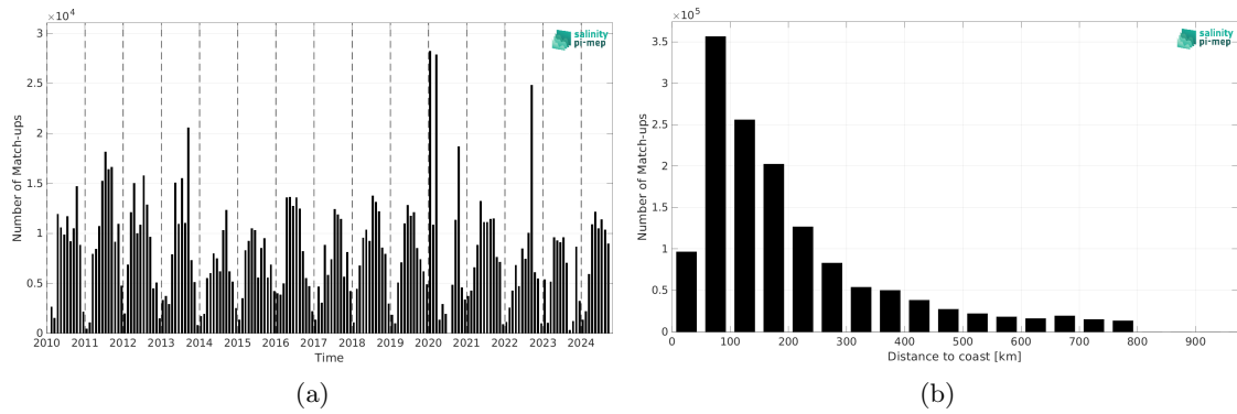
Figure 2: Number of match-ups between TSG (SAMOS) and SMOS SSS L3 v332 - 9 Days (CATDS-CPDC) SSS as a function of time (a) and as function of the distance to coast (b) over the SMOS coastal zone (<800km) 60N-60S Pi-MEP region and for the full satellite product period.
