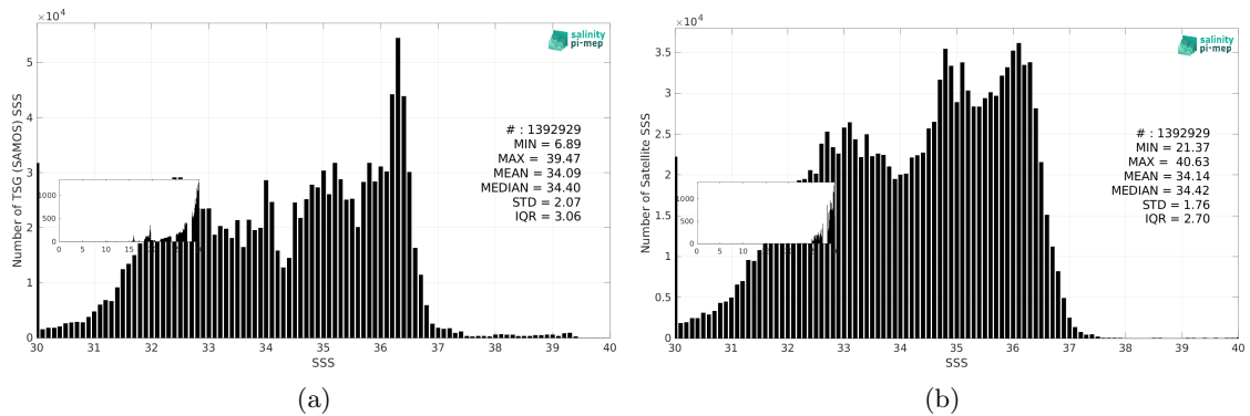
Figure 3: Histograms of SSS from TSG (SAMOS) (a) and SMOS SSS L3 v332 - 9 Days (CATDS-CPDC) (b) considering all match-up pairs per bins of 0.1 over the SMOS coastal zone (<800km) 60N-60S Pi-MEP region and for the full satellite product period.
