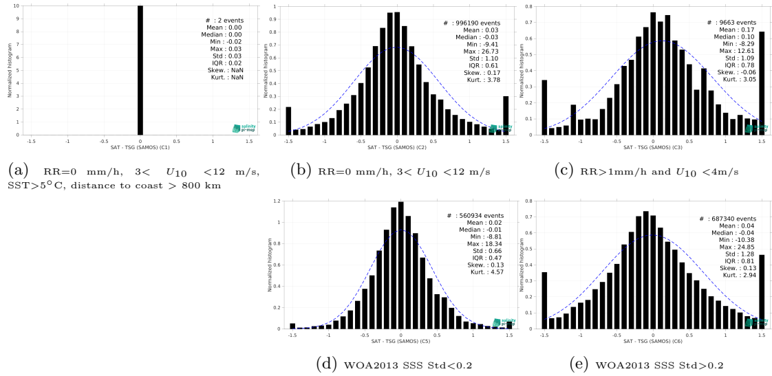
Figure 15: Normalized histogram of \Delta SSS (SMOS SSS L3 v332 - 9 Days (CATDS-CPDC) - TSG (SAMOS)) for 5 different subdatasets corresponding to: RR=0 mm/h, 3 < U_{10} < 12 m/s, SST > 5^\circ C , distance to coast > 800 km (a), RR=0 mm/h, 3 < U_{10} < 12 m/s (b), RR > 1 mm/h and U_{10} < 4 m/s (c), WOA2013 SSS Std < 0.2 (d), WOA2013 SSS Std > 0.2 (e).
