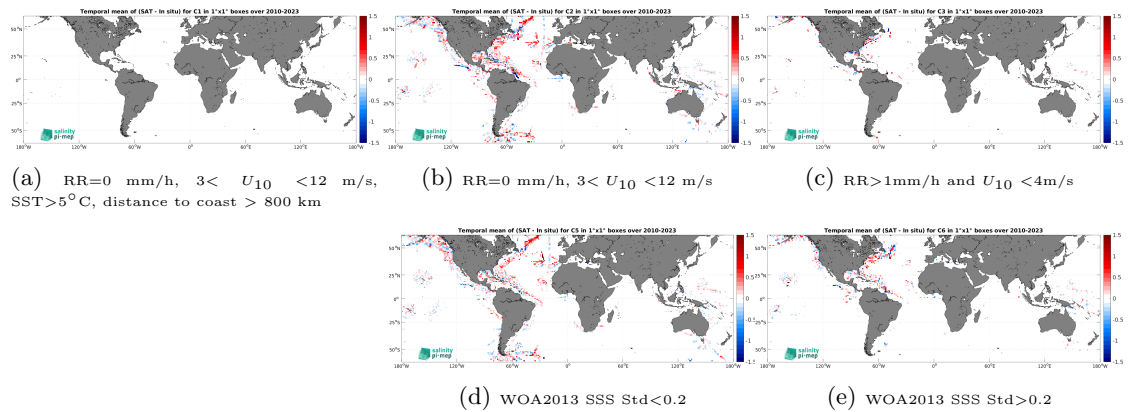
Figure 12: Temporal mean gridded over spatial boxes of size 1^\circ \times 1^\circ of \Delta\text{SSS} (SMOS SSS L3 v332 - 9 Days (CATDS-CPDC) - TSG (SAMOS)) for 5 different subdatasets corresponding to:RR=0 mm/h, 3 < U_{10} < 12 m/s, SST >5^\circ\text{C} , distance to coast > 800 km (a), RR=0 mm/h, 3 < U_{10} < 12 m/s (b), RR >1 mm/h and U_{10} < 4 m/s (c), WOA2013 SSS Std <0.2 (d), WOA2013 SSS Std >0.2 (e).
