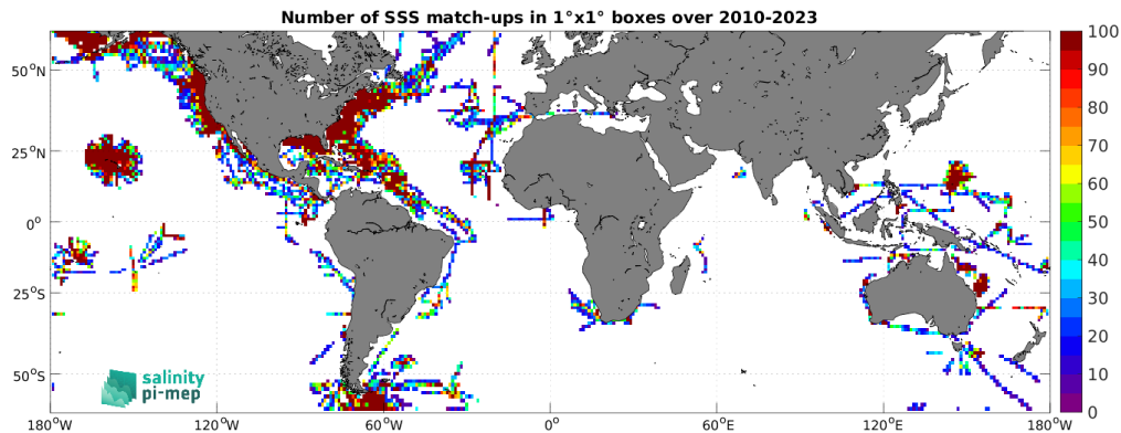
Figure 4: Number of SSS match-ups between TSG (SAMOS) SSS and the SMOS SSS L3 v332 - 9 Days (CATDS-CPDC) SSS product for the SMOS coastal zone (<800km) 60N-60S Pi-MEP region over 1^\circ \times 1^\circ boxes and for the full satellite product period.
