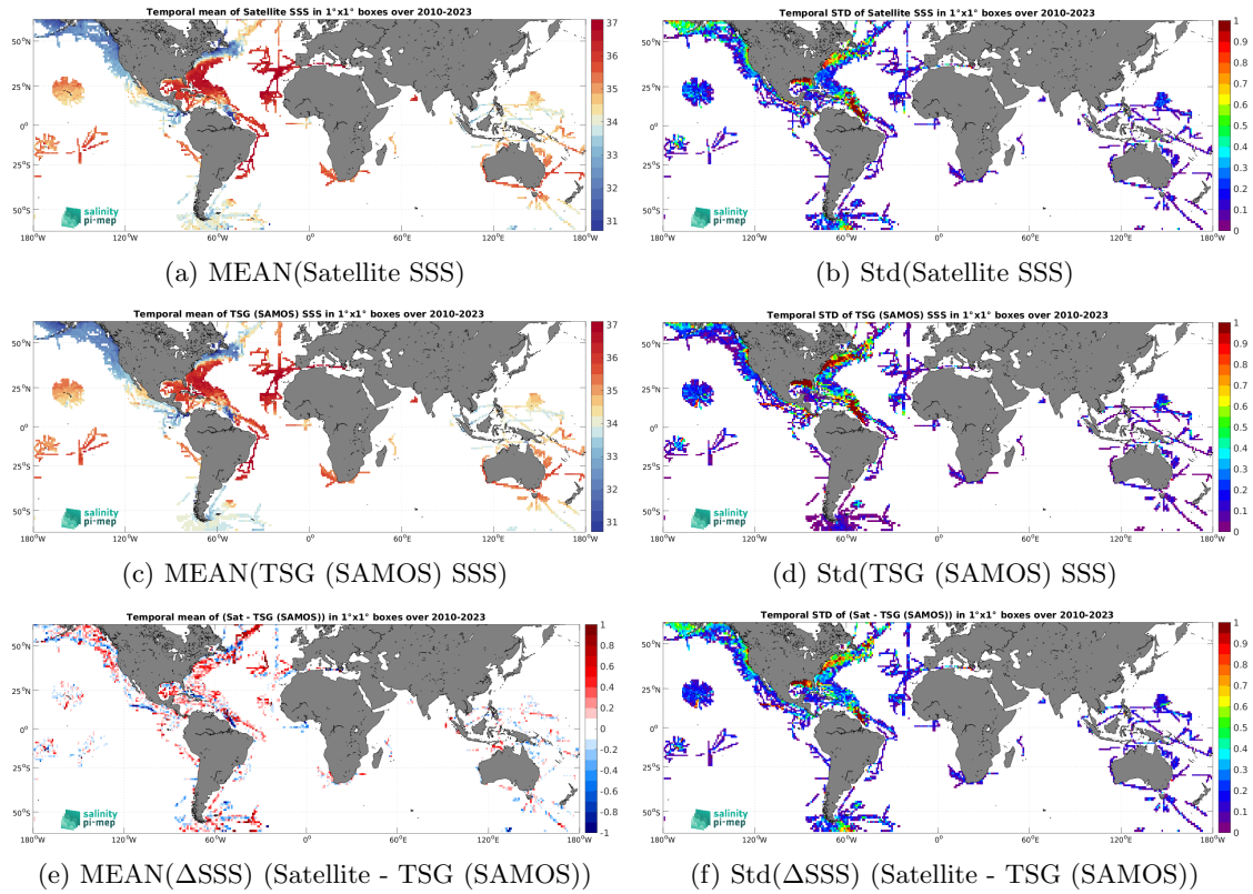
Figure 6: Temporal mean (left) and Std (right) of SSS from SMOS SSS L3 v332 - 9 Days (CATDS-CPDC) (top), TSG (SAMOS) (middle), and of \Delta SSS (Satellite - TSG (SAMOS)). Only match-up pairs are used to generate these maps.
