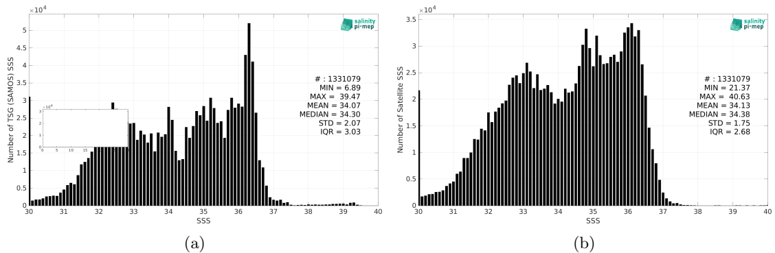
Figure 2: Histograms of SSS from TSG (SAMOS) (a) and SMOS SSS L3 v332 - 9 Days (CATDS-CPDC) (b) considering all match-up pairs per bins of 0.1 over the SMOS coastal zone (<800km) 60N-60S Pi-MEP region and for the full satellite product period.
