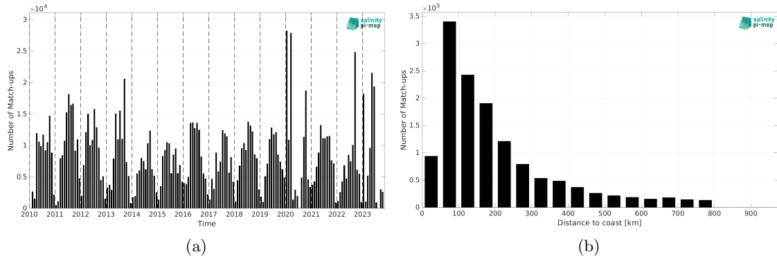
Figure 1: Number of match-ups between TSG (SAMOS) and SMOS SSS L3 v332 - 9 Days (CATDS-CPDC) SSS as a function of time (a) and as function of the distance to coast (b) over the SMOS coastal zone (<800km) 60N-60S Pi-MEP region and for the full satellite product period.
