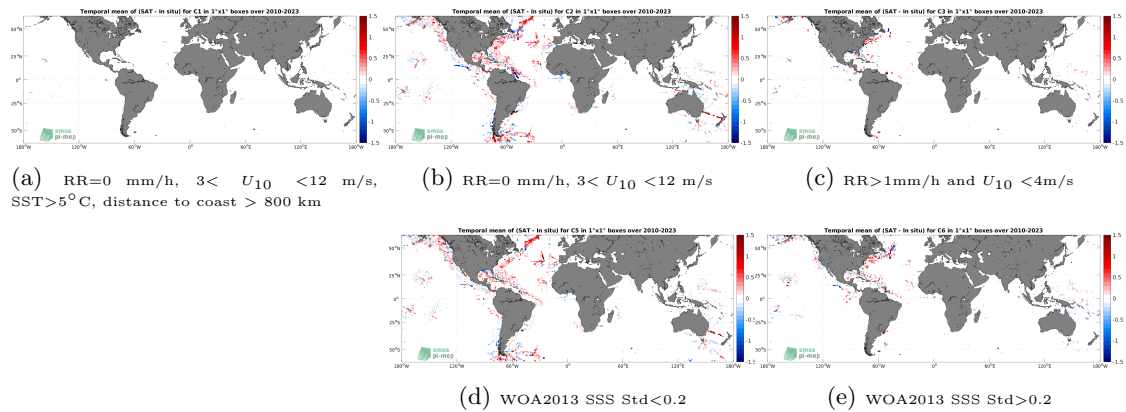
Figure 12: Temporal mean gridded over spatial boxes of size 1^\circ \times 1^\circ of \Delta SSS (SMOS SSS L3 v332 - 9 Days (CATDS-CPDC) - TSG (SAMOS)) for 5 different subdatasets corresponding to:RR=0 mm/h, 3 < U_{10} < 12 m/s, SST >5^\circ\text{C} , distance to coast > 800 km (a), RR=0 mm/h, 3 < U_{10} < 12 m/s (b), RR >1 mm/h and U_{10} < 4 m/s (c), WOA2013 SSS Std <0.2 (d), WOA2013 SSS Std >0.2 (e).
