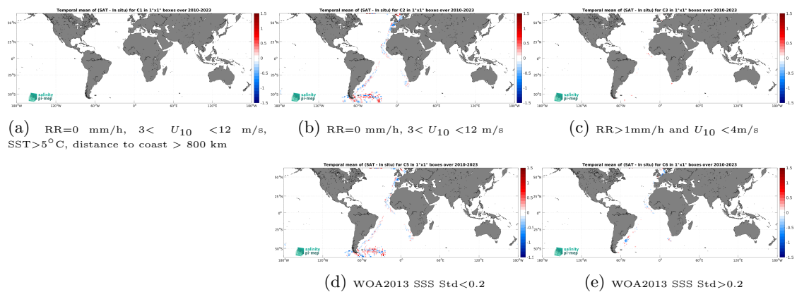
Figure 14: Temporal mean gridded over spatial boxes of size 1^\circ \times 1^\circ of \Delta SSS (SMOS SSS L3 v332 - 9 Days (CATDS-CPDC) - TSG (Polarstern)) for 5 different subdatasets corresponding to:RR=0 mm/h, 3 < U_{10} < 12 m/s, SST > 5^\circ\text{C} , distance to coast > 800 km (a), RR=0 mm/h, 3 < U_{10} < 12 m/s (b), RR > 1 mm/h and U_{10} < 4 m/s (c), WOA2013 SSS Std < 0.2 (d), WOA2013 SSS Std > 0.2 (e).
