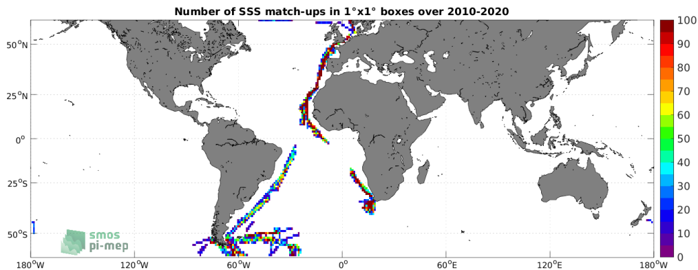
Figure 4: Number of SSS match-ups between TSG (Polarstern) SSS and the SMOS SSS L3 v332 - 9 Days (CATDS-CPDC) SSS product for the SMOS coastal zone (<800km) 60N-60S Pi-MEP region over 1^\circ \times 1^\circ boxes and for the full satellite product period.
