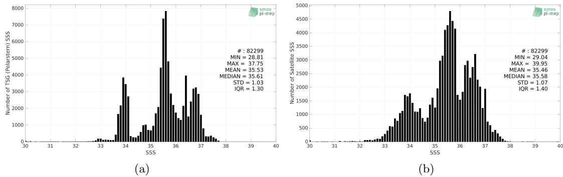
Figure 2: Histograms of SSS from TSG (Polarstern) (a) and SMOS SSS L3 v332 - 9 Days (CATDS-CPDC) (b) considering all match-up pairs per bins of 0.1 over the SMOS coastal zone ( <800\text{km} ) 60N-60S Pi-MEP region and for the full satellite product period.
