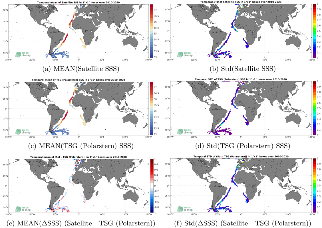
Figure 6: Temporal mean (left) and Std (right) of SSS from SMOS SSS L3 v332 - 9 Days (CATDS-CPDC) (top), TSG (Polarstern) (middle), and of \Delta SSS (Satellite - TSG (Polarstern)). Only match-up pairs are used to generate these maps.
