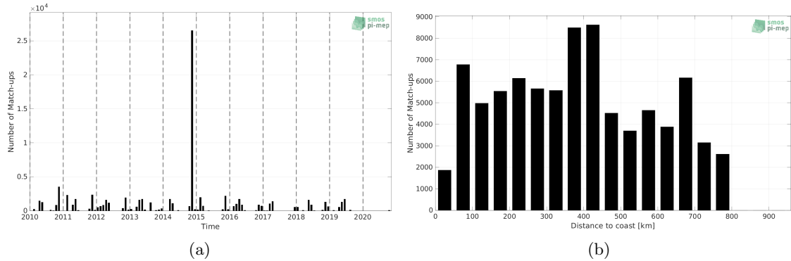
Figure 1: Number of match-ups between TSG (Polarstern) and SMOS SSS L3 v332 - 9 Days (CATDS-CPDC) SSS as a function of time (a) and as function of the distance to coast (b) over the SMOS coastal zone ( <800\text{km} ) 60N-60S Pi-MEP region and for the full satellite product period.
