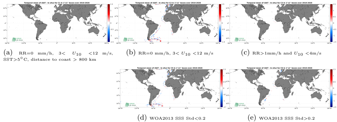
Figure 12: Temporal mean gridded over spatial boxes of size 1^\circ \times 1^\circ of \Delta SSS (SMOS SSS L3 v332 - 9 Days (CATDS-CPDC) - TSG (Polarstern)) for 5 different subdatasets corresponding to:RR=0 mm/h, 3 < U_{10} < 12 m/s, SST >5^\circ C, distance to coast > 800 km (a), RR=0 mm/h, 3 < U_{10} < 12 m/s (b), RR >1 mm/h and U_{10} < 4 m/s (c), WOA2013 SSS Std <0.2 (d), WOA2013 SSS Std >0.2 (e).
