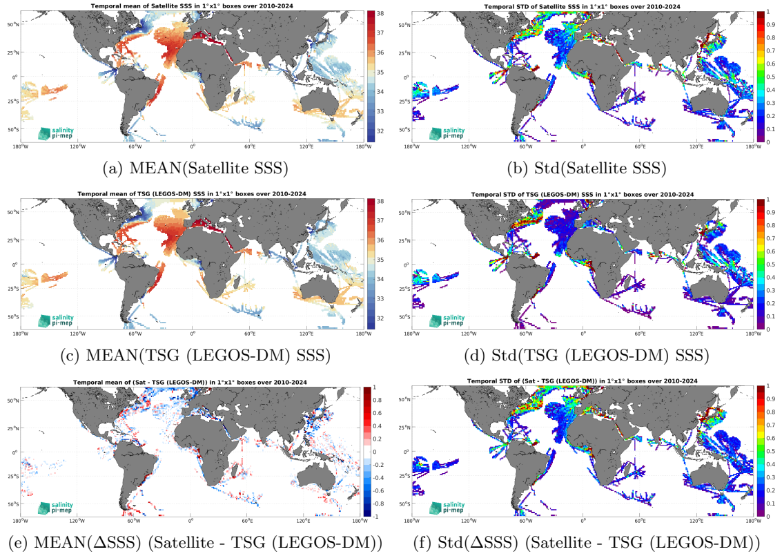
Figure 7: Temporal mean (left) and Std (right) of SSS from SMOS SSS L3 v332 - 9 Days (CATDS-CPDC) (top), TSG (LEGOS-DM) (middle), and of \Delta SSS (Satellite - TSG (LEGOS-DM)). Only match-up pairs are used to generate these maps.
