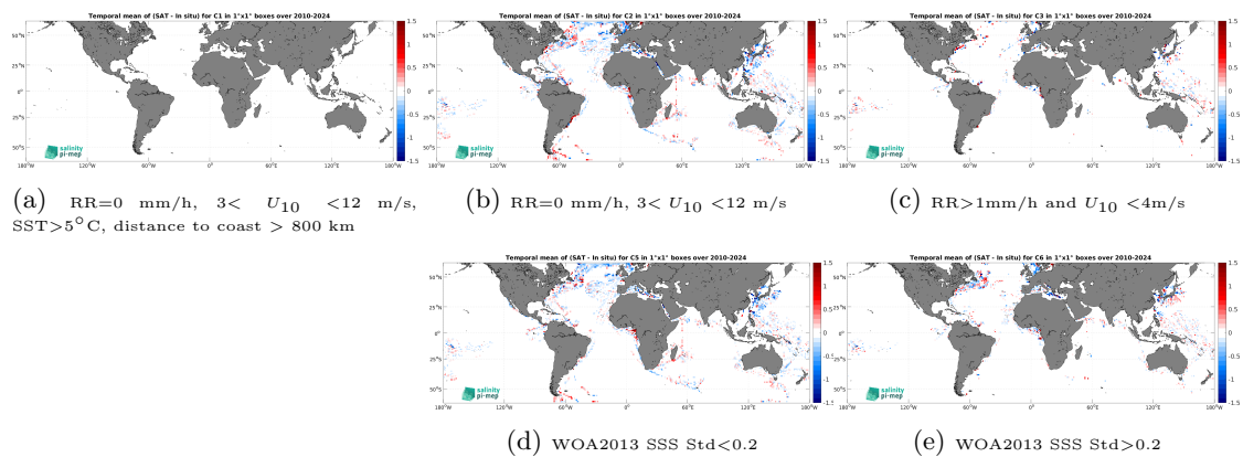
Figure 14: Temporal mean gridded over spatial boxes of size 1^\circ \times 1^\circ of \Delta\text{SSS} (SMOS SSS L3 v332 - 9 Days (CATDS-CPDC) - TSG (LEGOS-DM)) for 5 different subdatasets corresponding to:RR=0 mm/h, 3 < U_{10} < 12 m/s, SST >5^\circ\text{C} , distance to coast > 800 km (a), RR=0 mm/h, 3 < U_{10} < 12 m/s (b), RR >1 mm/h and U_{10} < 4 m/s (c), WOA2013 SSS Std <0.2 (d), WOA2013 SSS Std >0.2 (e).
