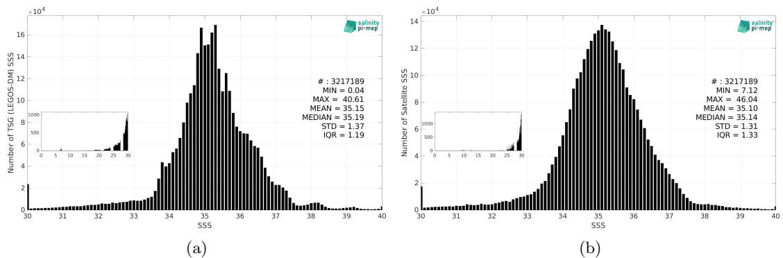
Figure 3: Histograms of SSS from TSG (LEGOS-DM) (a) and SMOS SSS L3 v332 - 9 Days (CATDS-CPDC) (b) considering all match-up pairs per bins of 0.1 over the SMOS coastal zone (<800km) 60N-60S Pi-MEP region and for the full satellite product period.
