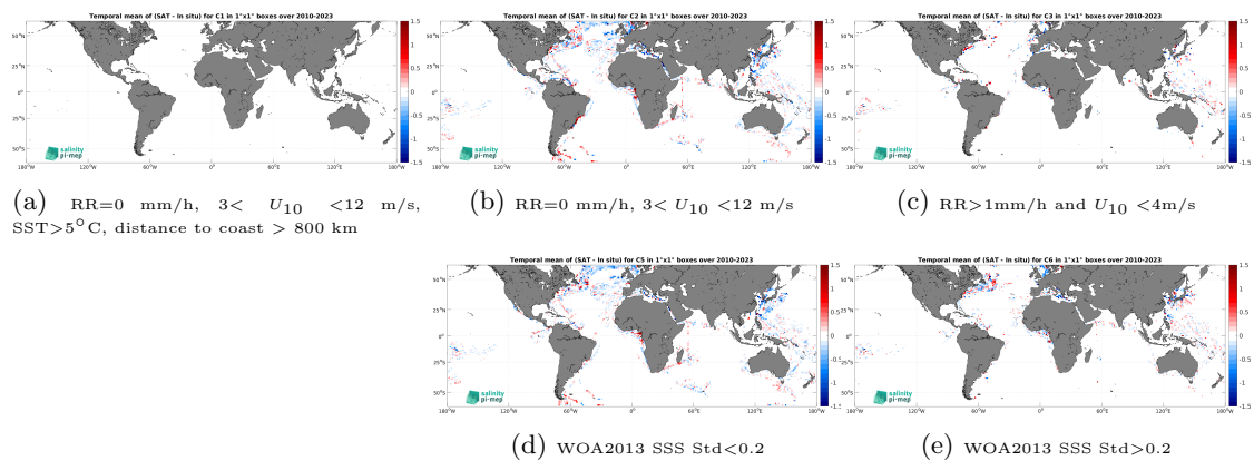
Figure 14: Temporal mean gridded over spatial boxes of size 1^\circ \times 1^\circ of \Delta SSS (SMOS SSS L3 v332 - 9 Days (CATDS-CPDC) - TSG (LEGOS-DM)) for 5 different subdatasets corresponding to:RR=0 mm/h, 3 < U_{10} < 12 m/s, SST >5^\circ\text{C} , distance to coast > 800 km (a), RR=0 mm/h, 3 < U_{10} < 12 m/s (b), RR >1 mm/h and U_{10} < 4 m/s (c), WOA2013 SSS Std <0.2 (d), WOA2013 SSS Std >0.2 (e).
