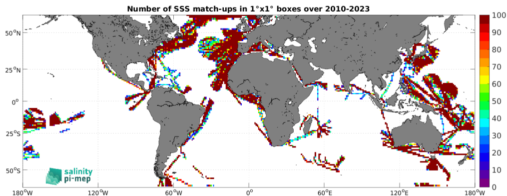
Figure 5: Number of SSS match-ups between TSG (LEGOS-DM) SSS and the SMOS SSS L3 v332 - 9 Days (CATDS-CPDC) SSS product for the SMOS coastal zone (<800km) 60N-60S Pi-MEP region over 1°x1° boxes and for the full satellite product period.
