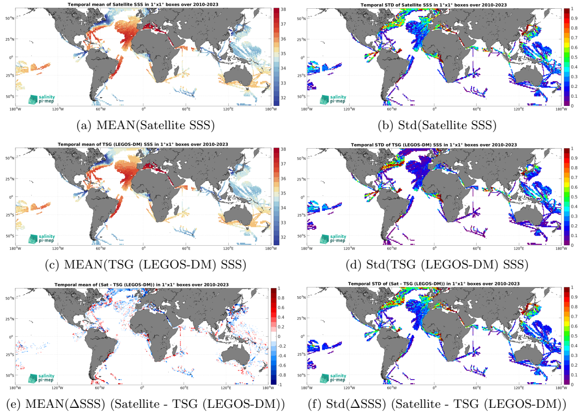
Figure 6: Temporal mean (left) and Std (right) of SSS from SMOS SSS L3 v332 - 9 Days (CATDS-CPDC) (top), TSG (LEGOS-DM) (middle), and of \Delta SSS (Satellite - TSG (LEGOS-DM)). Only match-up pairs are used to generate these maps.
