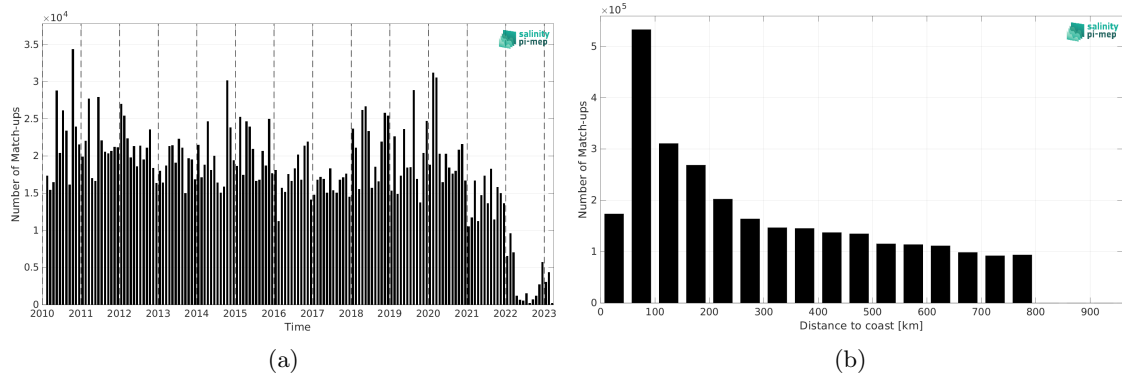
Figure 1: Number of match-ups between TSG (LEGOS-DM) and SMOS SSS L3 v332 - 9 Days (CATDS-CPDC) SSS as a function of time (a) and as function of the distance to coast (b) over the SMOS coastal zone (<800km) 60N-60S Pi-MEP region and for the full satellite product period.
