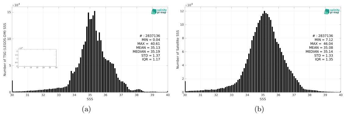
Figure 2: Histograms of SSS from TSG (LEGOS-DM) (a) and SMOS SSS L3 v332 - 9 Days (CATDS-CPDC) (b) considering all match-up pairs per bins of 0.1 over the SMOS coastal zone (<800km) 60N-60S Pi-MEP region and for the full satellite product period.
