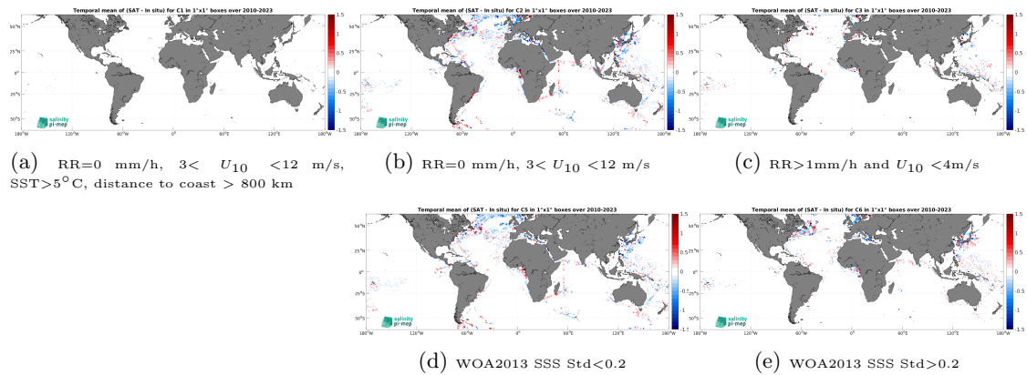
Figure 12: Temporal mean gridded over spatial boxes of size 1^\circ \times 1^\circ of \Delta SSS (SMOS SSS L3 v332 - 9 Days (CATDS-CPDC) - TSG (LEGOS-DM)) for 5 different subdatasets corresponding to:RR=0 mm/h, 3 < U_{10} < 12 m/s, SST >5^\circ C, distance to coast > 800 km (a), RR=0 mm/h, 3 < U_{10} < 12 m/s (b), RR >1 mm/h and U_{10} < 4 m/s (c), WOA2013 SSS Std <0.2 (d), WOA2013 SSS Std >0.2 (e).
