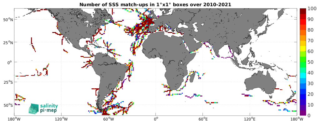
Figure 5: Number of SSS match-ups between TSG (GOSUD-Sailing-ship) SSS and the SMOS SSS L3 v332 - 9 Days (CATDS-CPDC) SSS product for the SMOS coastal zone (<800km) 60N-60S Pi-MEP region over 1^\circ \times 1^\circ boxes and for the full satellite product period.
