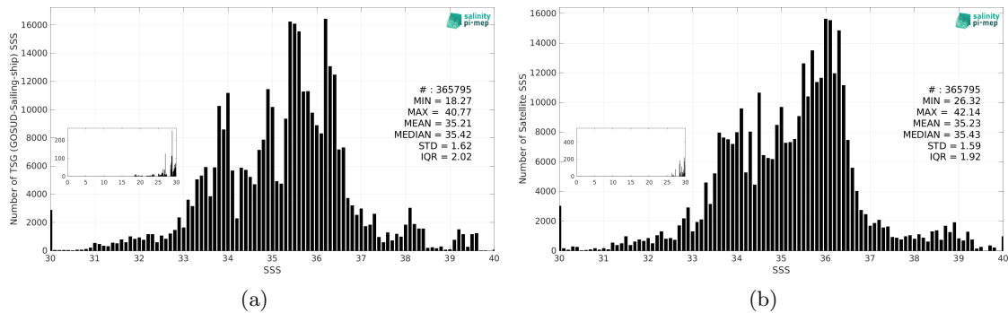
Figure 3: Histograms of SSS from TSG (GOSUD-Sailing-ship) (a) and SMOS SSS L3 v332 - 9 Days (CATDS-CPDC) (b) considering all match-up pairs per bins of 0.1 over the SMOS coastal zone (<800km) 60N-60S Pi-MEP region and for the full satellite product period.
