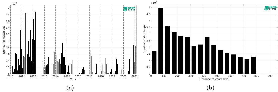
Figure 2: Number of match-ups between TSG (GOSUD-Sailing-ship) and SMOS SSS L3 v332 - 9 Days (CATDS-CPDC) SSS as a function of time (a) and as function of the distance to coast (b) over the SMOS coastal zone (<800km) 60N-60S Pi-MEP region and for the full satellite product period.
