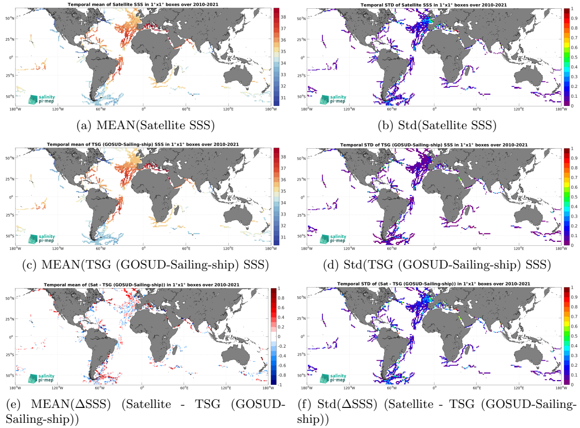
Figure 7: Temporal mean (left) and Std (right) of SSS from SMOS SSS L3 v332 - 9 Days (CATDS-CPDC) (top), TSG (GOSUD-Sailing-ship) (middle), and of \Delta SSS (Satellite - TSG (GOSUD-Sailing-ship)). Only match-up pairs are used to generate these maps.
