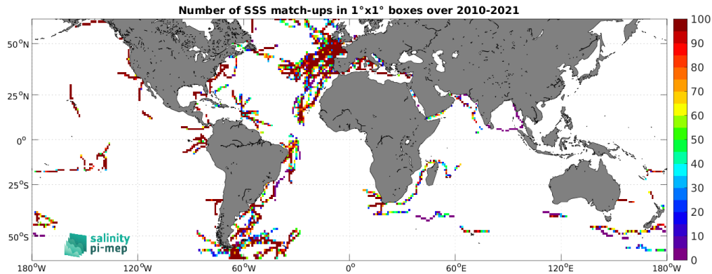
Figure 5: Number of SSS match-ups between TSG (GOSUD-Sailing-ship) SSS and the SMOS SSS L3 v332 - 9 Days (CATDS-CPDC) SSS product for the SMOS coastal zone ( <800\text{km} ) 60\text{N} - 60\text{S} Pi-MEP region over 1^\circ \times 1^\circ boxes and for the full satellite product period.
