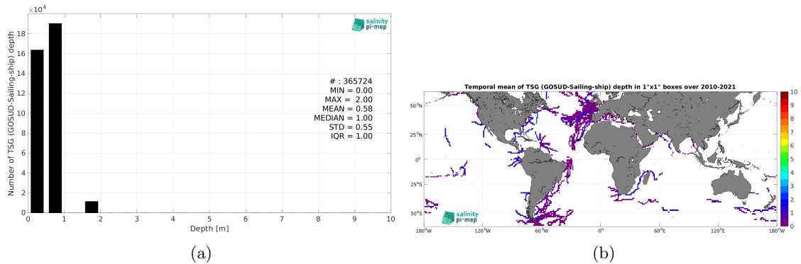
Figure 4: Histograms of the depth of the upper level SSS measurements from TSG (GOSUD-Sailing-ship) in the Match-up DataBase for the SMOS coastal zone ( <800\text{km} ) 60\text{N} - 60\text{S} Pi-MEP region (a) and temporal mean spatial distribution of pressure of the in situ SSS data over 1^\circ \times 1^\circ boxes and for the full satellite product period (b).
