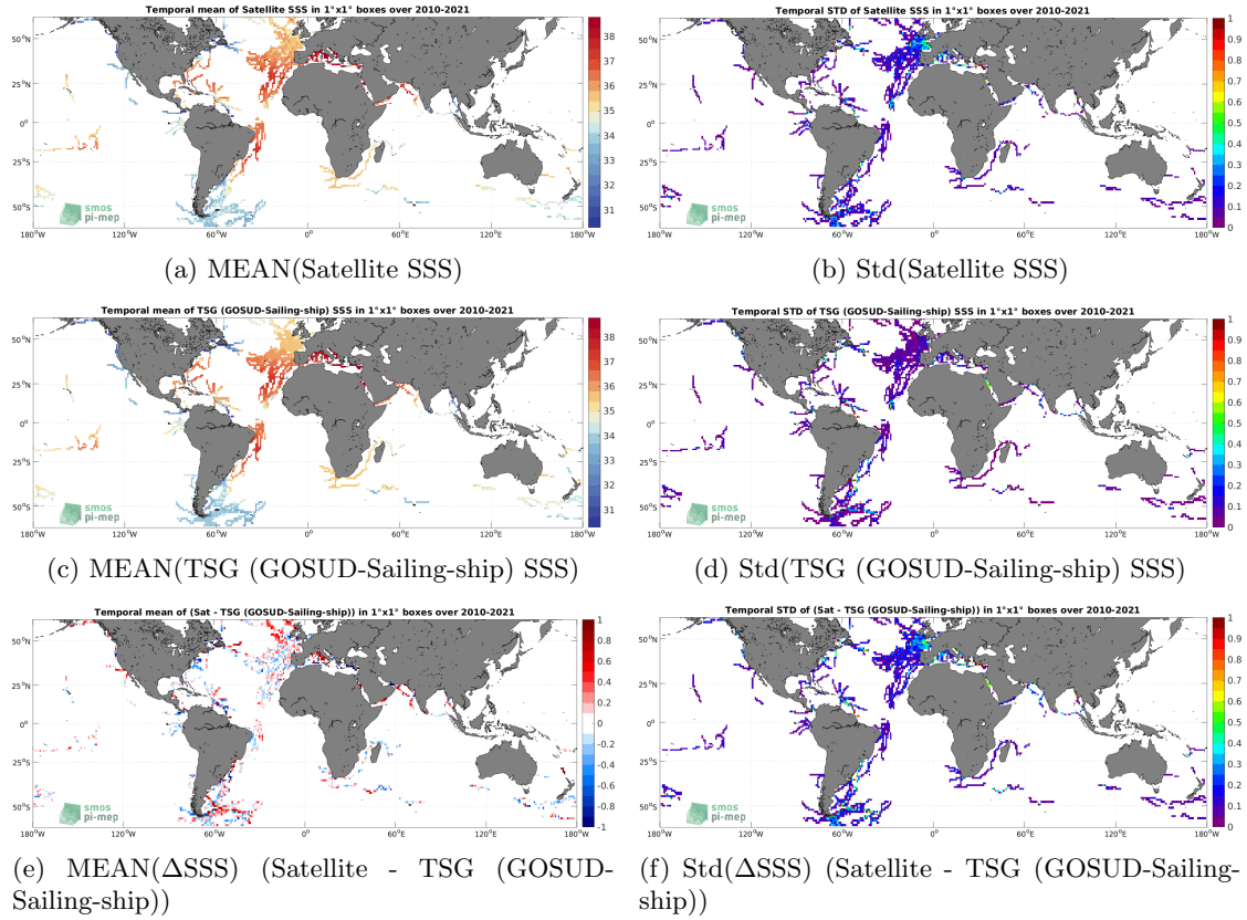
Figure 6: Temporal mean (left) and Std (right) of SSS from SMOS SSS L3 v332 - 9 Days (CATDS-CPDC) (top), TSG (GOSUD-Sailing-ship) (middle), and of \Delta SSS (Satellite - TSG (GOSUD-Sailing-ship)). Only match-up pairs are used to generate these maps.
