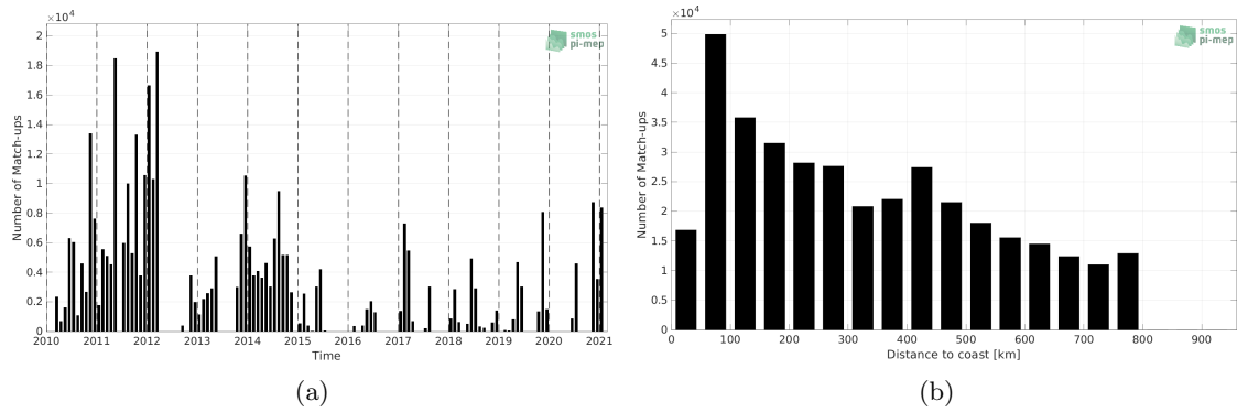
Figure 1: Number of match-ups between TSG (GOSUD-Sailing-ship) and SMOS SSS L3 v332 - 9 Days (CATDS-CPDC) SSS as a function of time (a) and as function of the distance to coast (b) over the SMOS coastal zone (<800km) 60N-60S Pi-MEP region and for the full satellite product period.
