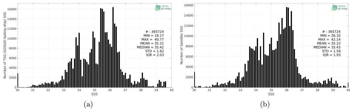
Figure 2: Histograms of SSS from TSG (GOSUD-Sailing-ship) (a) and SMOS SSS L3 v332 - 9 Days (CATDS-CPDC) (b) considering all match-up pairs per bins of 0.1 over the SMOS coastal zone (<800km) 60N-60S Pi-MEP region and for the full satellite product period.
