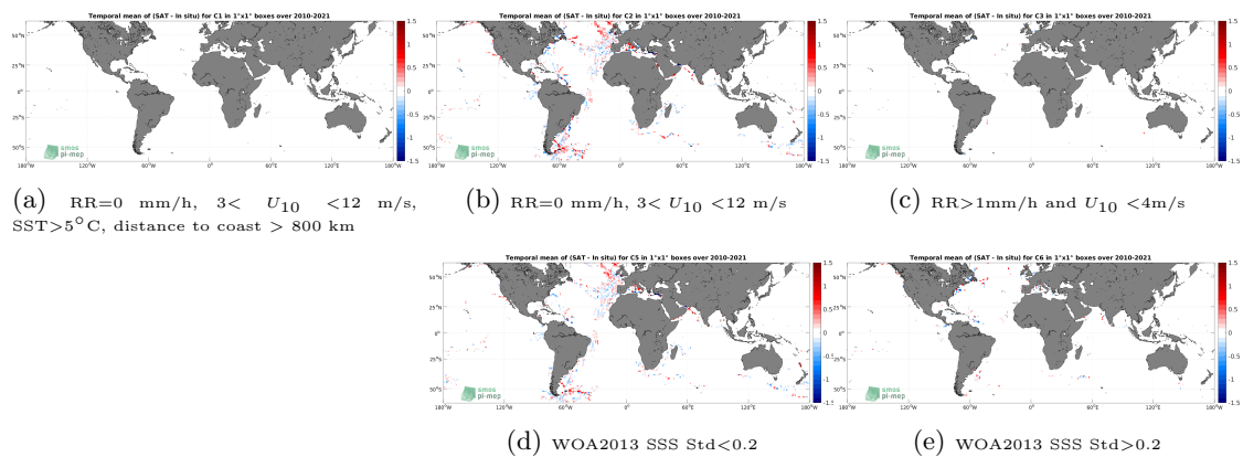
Figure 12: Temporal mean gridded over spatial boxes of size 1^\circ \times 1^\circ of \Delta SSS (SMOS SSS L3 v332 - 9 Days (CATDS-CPDC) - TSG (GOSUD-Sailing-ship)) for 5 different subdatasets corresponding to:RR=0 mm/h, 3 < U_{10} < 12 m/s, SST >5^\circ C, distance to coast > 800 km (a), RR=0 mm/h, 3 < U_{10} < 12 m/s (b), RR >1 mm/h and U_{10} < 4 m/s (c), WOA2013 SSS Std <0.2 (d), WOA2013 SSS Std >0.2 (e).
