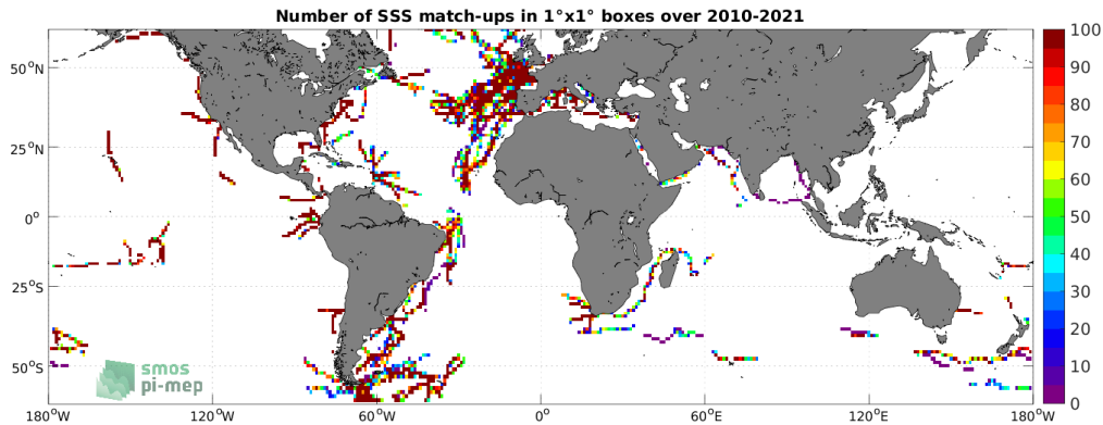
Figure 4: Number of SSS match-ups between TSG (GOSUD-Sailing-ship) SSS and the SMOS SSS L3 v332 - 9 Days (CATDS-CPDC) SSS product for the SMOS coastal zone (<800km) 60N-60S Pi-MEP region over 1^\circ \times 1^\circ boxes and for the full satellite product period.
