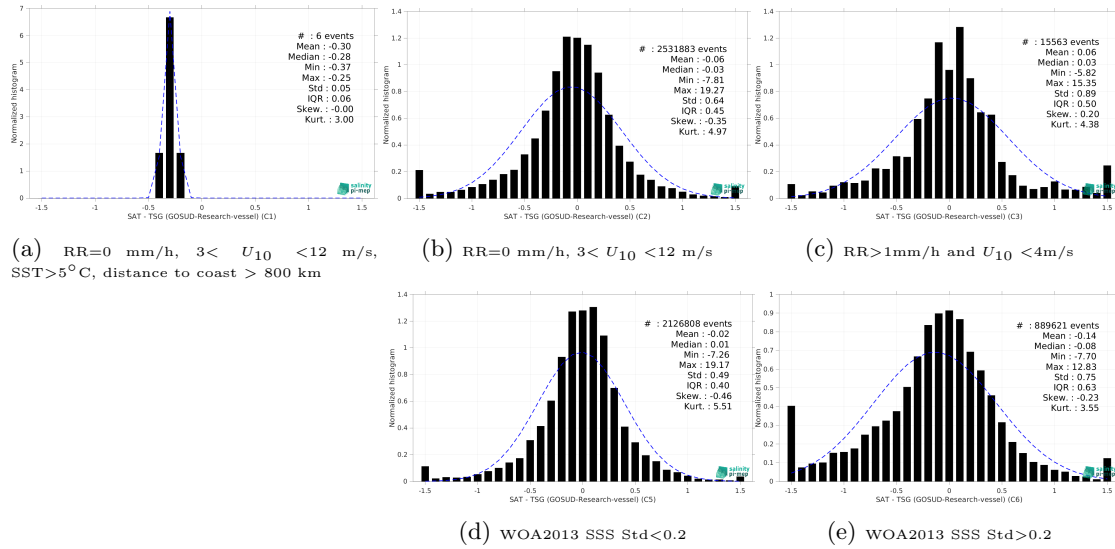
Figure 15: Normalized histogram of \Delta\text{SSS} (SMOS SSS L3 v332 - 9 Days (CATDS-CPDC) - TSG (GOSUD-Research-vessel)) for 5 different subdatasets corresponding to: RR=0 mm/h, 3 < U_{10} < 12 m/s, SST > 5^\circ\text{C} , distance to coast > 800 km (a), RR=0 mm/h, 3 < U_{10} < 12 m/s (b), RR > 1\text{mm/h} and U_{10} < 4\text{m/s} (c), WOA2013 SSS Std < 0.2 (d), WOA2013 SSS Std > 0.2 (e).
