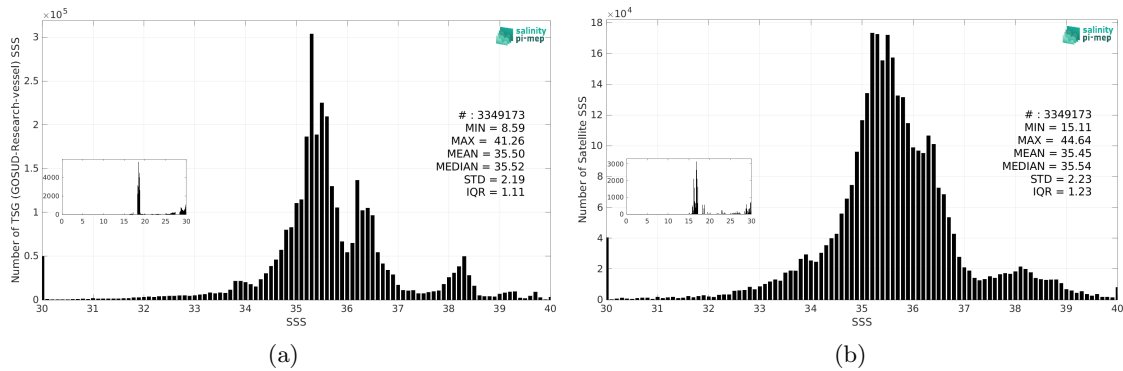
Figure 3: Histograms of SSS from TSG (GOSUD-Research-vessel) (a) and SMOS SSS L3 v332 - 9 Days (CATDS-CPDC) (b) considering all match-up pairs per bins of 0.1 over the SMOS coastal zone (<800km) 60N-60S Pi-MEP region and for the full satellite product period.
