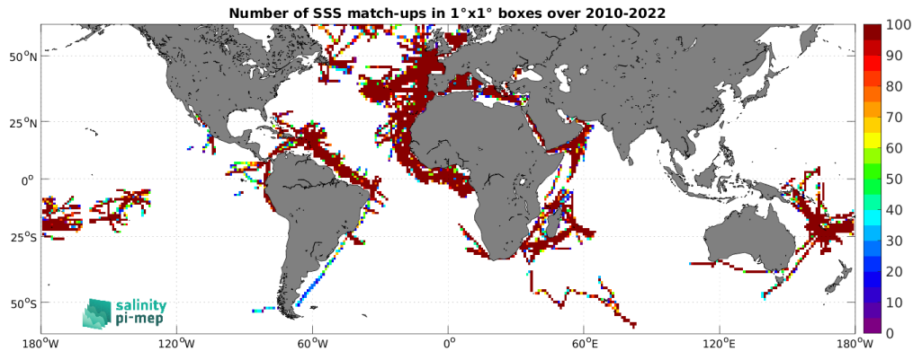
Figure 5: Number of SSS match-ups between TSG (GOSUD-Research-vessel) SSS and the SMOS SSS L3 v332 - 9 Days (CATDS-CPDC) SSS product for the SMOS coastal zone (<800km) 60N-60S Pi-MEP region over 1°×1° boxes and for the full satellite product period.
