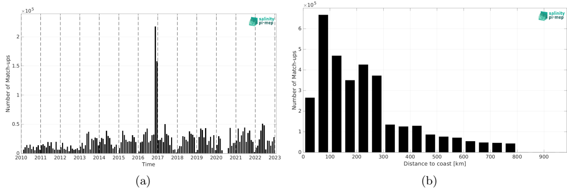
Figure 2: Number of match-ups between TSG (GOSUD-Research-vessel) and SMOS SSS L3 v332 - 9 Days (CATDS-CPDC) SSS as a function of time (a) and as function of the distance to coast (b) over the SMOS coastal zone (<800km) 60N-60S Pi-MEP region and for the full satellite product period.
