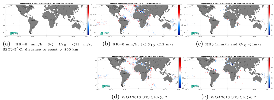
Figure 14: Temporal mean gridded over spatial boxes of size 1^\circ \times 1^\circ of \Delta SSS (SMOS SSS L3 v332 - 9 Days (CATDS-CPDC) - TSG (GOSUD-Research-vessel)) for 5 different subdatasets corresponding to:RR=0 mm/h, 3 < U_{10} < 12 m/s, SST >5^\circ\text{C} , distance to coast > 800 km (a), RR=0 mm/h, 3 < U_{10} < 12 m/s (b), RR >1 mm/h and U_{10} < 4 m/s (c), WOA2013 SSS Std <0.2 (d), WOA2013 SSS Std >0.2 (e).
