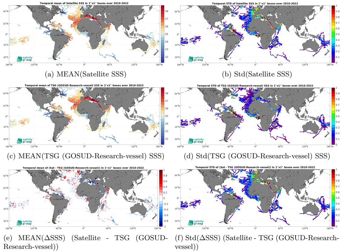
Figure 7: Temporal mean (left) and Std (right) of SSS from SMOS SSS L3 v332 - 9 Days (CATDS-CPDC) (top), TSG (GOSUD-Research-vessel) (middle), and of \Delta SSS (Satellite - TSG (GOSUD-Research-vessel)). Only match-up pairs are used to generate these maps.
