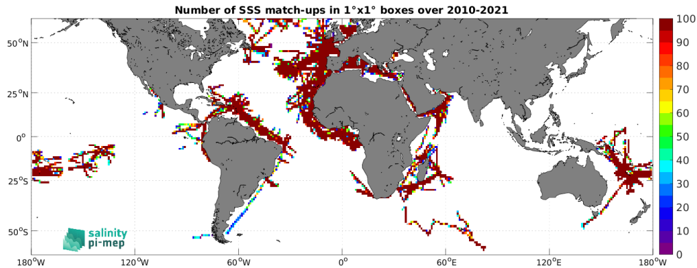
Figure 5: Number of SSS match-ups between TSG (GOSUD-Research-vessel) SSS and the SMOS SSS L3 v332 - 9 Days (CATDS-CPDC) SSS product for the SMOS coastal zone ( <800\text{km} ) 60N-60S Pi-MEP region over 1^\circ \times 1^\circ boxes and for the full satellite product period.
