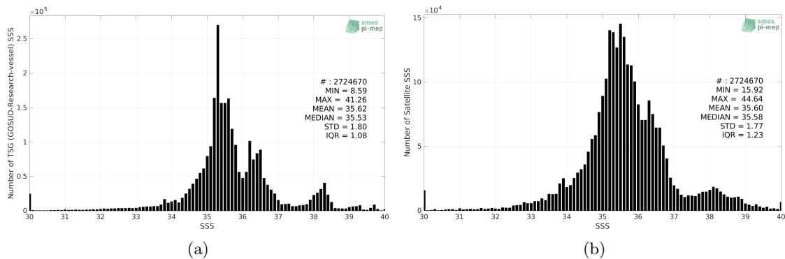
Figure 2: Histograms of SSS from TSG (GOSUD-Research-vessel) (a) and SMOS SSS L3 v332 - 9 Days (CATDS-CPDC) (b) considering all match-up pairs per bins of 0.1 over the SMOS coastal zone (<800km) 60N-60S Pi-MEP region and for the full satellite product period.
