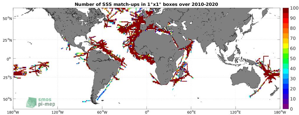
Figure 4: Number of SSS match-ups between TSG (GOSUD-Research-vessel) SSS and the SMOS SSS L3 v332 - 9 Days (CATDS-CPDC) SSS product for the SMOS coastal zone (<800km) 60N-60S Pi-MEP region over 1^\circ \times 1^\circ boxes and for the full satellite product period.
