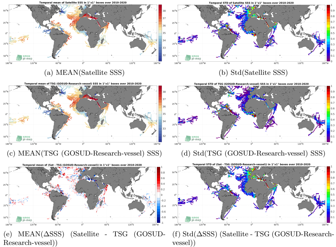
Figure 6: Temporal mean (left) and Std (right) of SSS from SMOS SSS L3 v332 - 9 Days (CATDS-CPDC) (top), TSG (GOSUD-Research-vessel) (middle), and of \Delta SSS (Satellite - TSG (GOSUD-Research-vessel)). Only match-up pairs are used to generate these maps.
