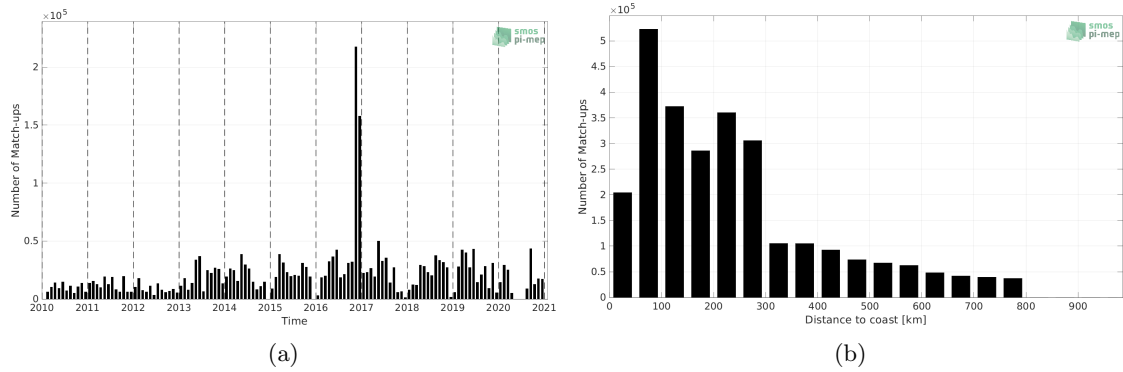
Figure 1: Number of match-ups between TSG (GOSUD-Research-vessel) and SMOS SSS L3 v332 - 9 Days (CATDS-CPDC) SSS as a function of time (a) and as function of the distance to coast (b) over the SMOS coastal zone (<800km) 60N-60S Pi-MEP region and for the full satellite product period.
