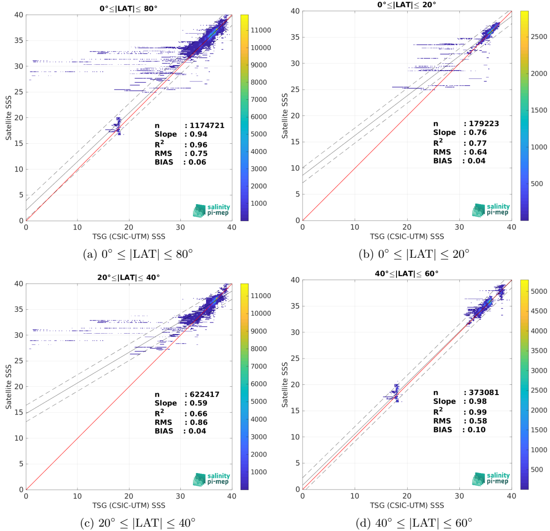
Figure 10: Contour maps of the concentration of SMOS SSS L3 v332 - 9 Days (CATDS-CPDC) SSS (y-axis) versus TSG (CSIC-UTM) SSS (x-axis) at match-up pairs for different latitude bands. For each plot, the red line shows x=y . The black thin and dashed lines indicate a linear fit through the data cloud and the \pm 95\% confidence levels, respectively. The number match-up pairs n , the slope and R^2 coefficient of the linear fit, the root mean square (RMS) and the mean bias between satellite and in situ data are indicated for each latitude band in each plots.
