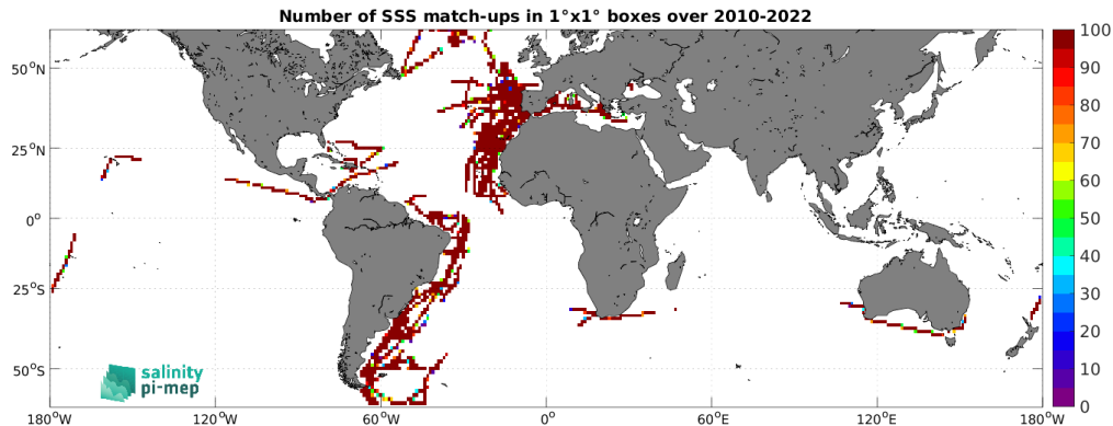
Figure 5: Number of SSS match-ups between TSG (CSIC-UTM) SSS and the SMOS SSS L3 v332 - 9 Days (CATDS-CPDC) SSS product for the SMOS coastal zone (<800km) 60N-60S Pi-MEP region over 1^\circ \times 1^\circ boxes and for the full satellite product period.
