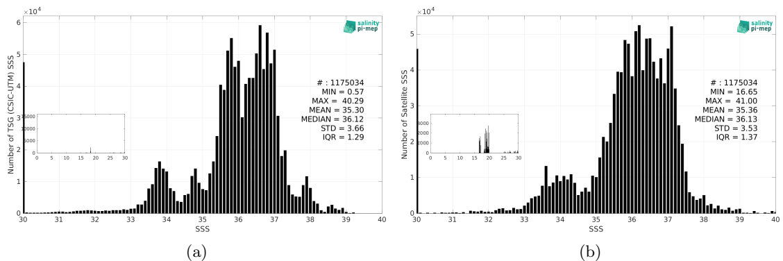
Figure 3: Histograms of SSS from TSG (CSIC-UTM) (a) and SMOS SSS L3 v332 - 9 Days (CATDS-CPDC) (b) considering all match-up pairs per bins of 0.1 over the SMOS coastal zone (<800km) 60N-60S Pi-MEP region and for the full satellite product period.
