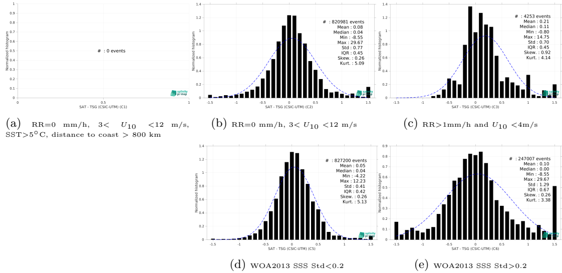
Figure 15: Normalized histogram of \Delta SSS (SMOS SSS L3 v332 - 9 Days (CATDS-CPDC) - TSG (CSIC-UTM)) for 5 different subdatasets corresponding to: RR=0 mm/h, 3 < U_{10} < 12 m/s, SST > 5°C, distance to coast > 800 km (a), RR=0 mm/h, 3 < U_{10} < 12 m/s (b), RR > 1mm/h and U_{10} < 4 m/s (c), WOA2013 SSS Std < 0.2 (d), WOA2013 SSS Std > 0.2 (e).
