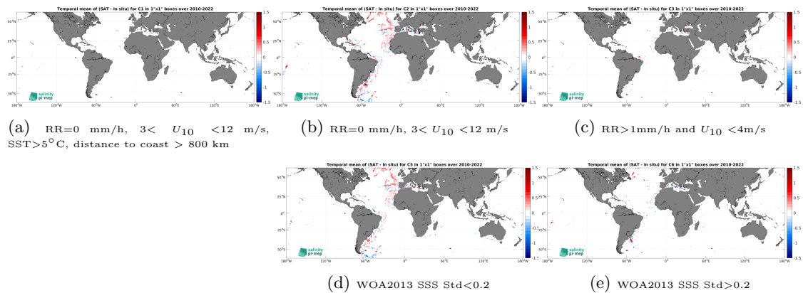
Figure 14: Temporal mean gridded over spatial boxes of size 1^\circ \times 1^\circ of \Delta SSS (SMOS SSS L3 v332 - 9 Days (CATDS-CPDC) - TSG (CSIC-UTM)) for 5 different subdatasets corresponding to:RR=0 mm/h, 3 < U_{10} < 12 m/s, SST >5^\circ\text{C} , distance to coast > 800 km (a), RR=0 mm/h, 3 < U_{10} < 12 m/s (b), RR >1 mm/h and U_{10} < 4 m/s (c), WOA2013 SSS Std <0.2 (d), WOA2013 SSS Std >0.2 (e).
