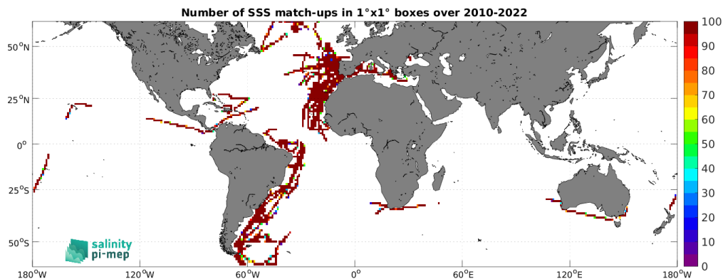
Figure 4: Number of SSS match-ups between TSG (CSIC-UTM) SSS and the SMOS SSS L3 v332 - 9 Days (CATDS-CPDC) SSS product for the SMOS coastal zone (<800km) 60N-60S Pi-MEP region over 1^\circ \times 1^\circ boxes and for the full satellite product period.
