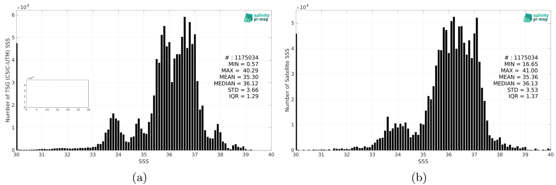
Figure 2: Histograms of SSS from TSG (CSIC-UTM) (a) and SMOS SSS L3 v332 - 9 Days (CATDS-CPDC) (b) considering all match-up pairs per bins of 0.1 over the SMOS coastal zone (<800km) 60N-60S Pi-MEP region and for the full satellite product period.
