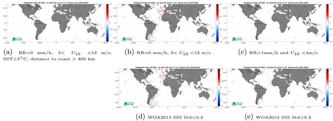
Figure 12: Temporal mean gridded over spatial boxes of size 1^\circ \times 1^\circ of \Delta SSS (SMOS SSS L3 v332 - 9 Days (CATDS-CPDC) - TSG (CSIC-UTM)) for 5 different subdatasets corresponding to:RR=0 mm/h, 3 < U_{10} < 12 m/s, SST >5^\circ C, distance to coast > 800 km (a), RR=0 mm/h, 3 < U_{10} < 12 m/s (b), RR >1 mm/h and U_{10} < 4 m/s (c), WOA2013 SSS Std <0.2 (d), WOA2013 SSS Std >0.2 (e).
