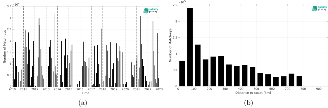
Figure 1: Number of match-ups between TSG (CSIC-UTM) and SMOS SSS L3 v332 - 9 Days (CATDS-CPDC) SSS as a function of time (a) and as function of the distance to coast (b) over the SMOS coastal zone (<800km) 60N-60S Pi-MEP region and for the full satellite product period.
