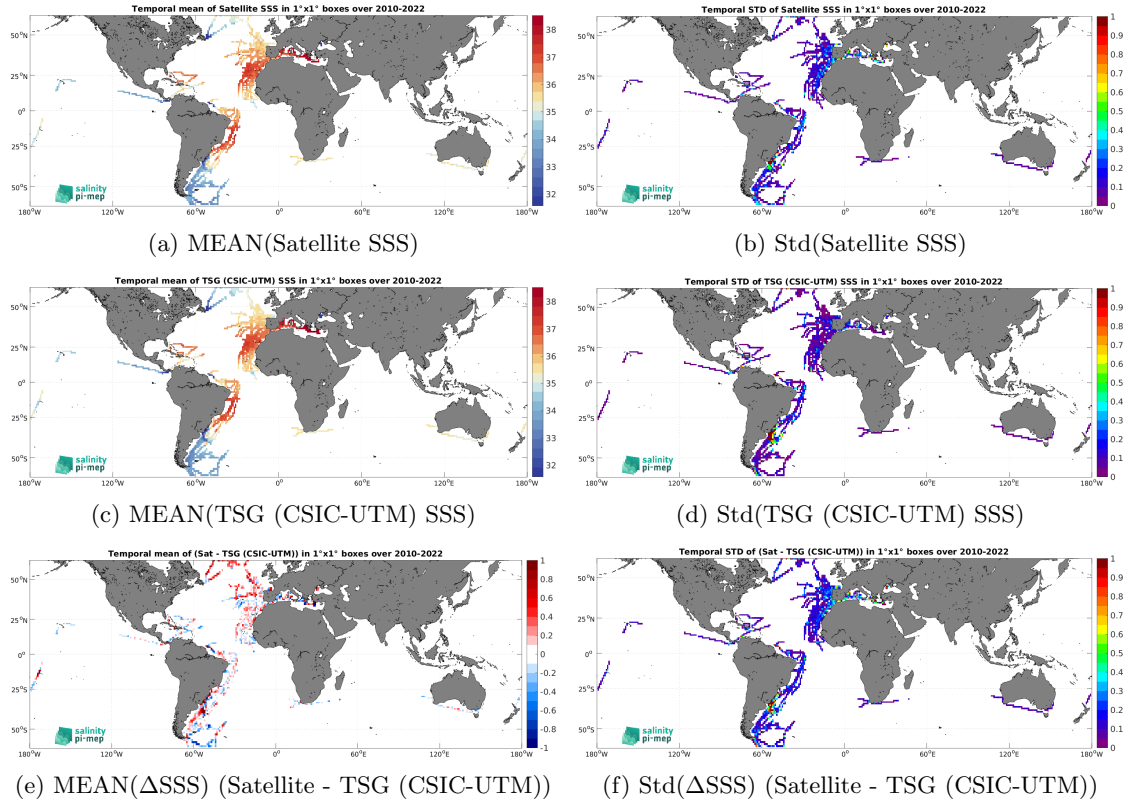
Figure 6: Temporal mean (left) and Std (right) of SSS from SMOS SSS L3 v332 - 9 Days (CATDS-CPDC) (top), TSG (CSIC-UTM) (middle), and of \Delta SSS (Satellite - TSG (CSIC-UTM)). Only match-up pairs are used to generate these maps.
