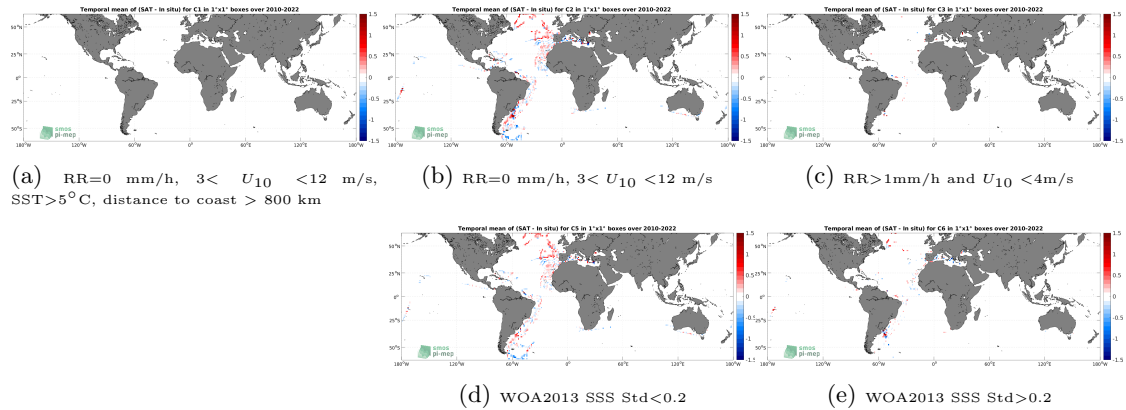
Figure 12: Temporal mean gridded over spatial boxes of size 1^\circ \times 1^\circ of \Delta\text{SSS} (SMOS SSS L3 v332 - 9 Days (CATDS-CPDC) - TSG (CSIC-UTM)) for 5 different subdatasets corresponding to:RR=0 mm/h, 3 < U_{10} < 12 m/s, SST >5^\circ\text{C} , distance to coast > 800 km (a), RR=0 mm/h, 3 < U_{10} < 12 m/s (b), RR >1 mm/h and U_{10} < 4 m/s (c), WOA2013 SSS Std <0.2 (d), WOA2013 SSS Std >0.2 (e).
