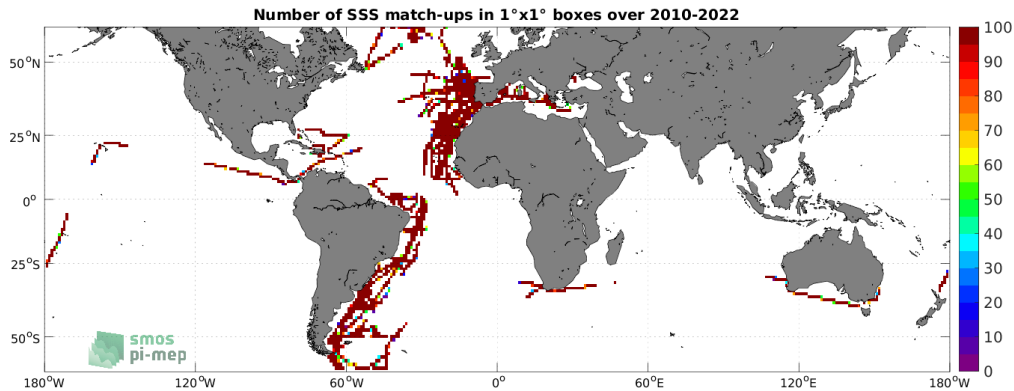
Figure 4: Number of SSS match-ups between TSG (CSIC-UTM) SSS and the SMOS SSS L3 v332 - 9 Days (CATDS-CPDC) SSS product for the SMOS coastal zone (<800km) 60N-60S Pi-MEP region over 1°×1° boxes and for the full satellite product period.
