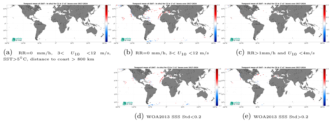
Figure 14: Temporal mean gridded over spatial boxes of size 1^\circ \times 1^\circ of \Delta SSS (SMOS SSS L3 v332 - 9 Days (CATDS-CPDC) - Saildrone) for 5 different subdatasets corresponding to:RR=0 mm/h, 3 < U_{10} < 12 m/s, SST >5^\circ\text{C} , distance to coast > 800 km (a), RR=0 mm/h, 3 < U_{10} < 12 m/s (b), RR >1 mm/h and U_{10} < 4 m/s (c), WOA2013 SSS Std <0.2 (d), WOA2013 SSS Std >0.2 (e).
