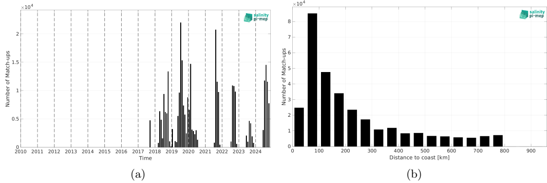
Figure 2: Number of match-ups between Saildrone and SMOS SSS L3 v332 - 9 Days (CATDS-CPDC) SSS as a function of time (a) and as function of the distance to coast (b) over the SMOS coastal zone (<800km) 60N-60S Pi-MEP region and for the full satellite product period.
