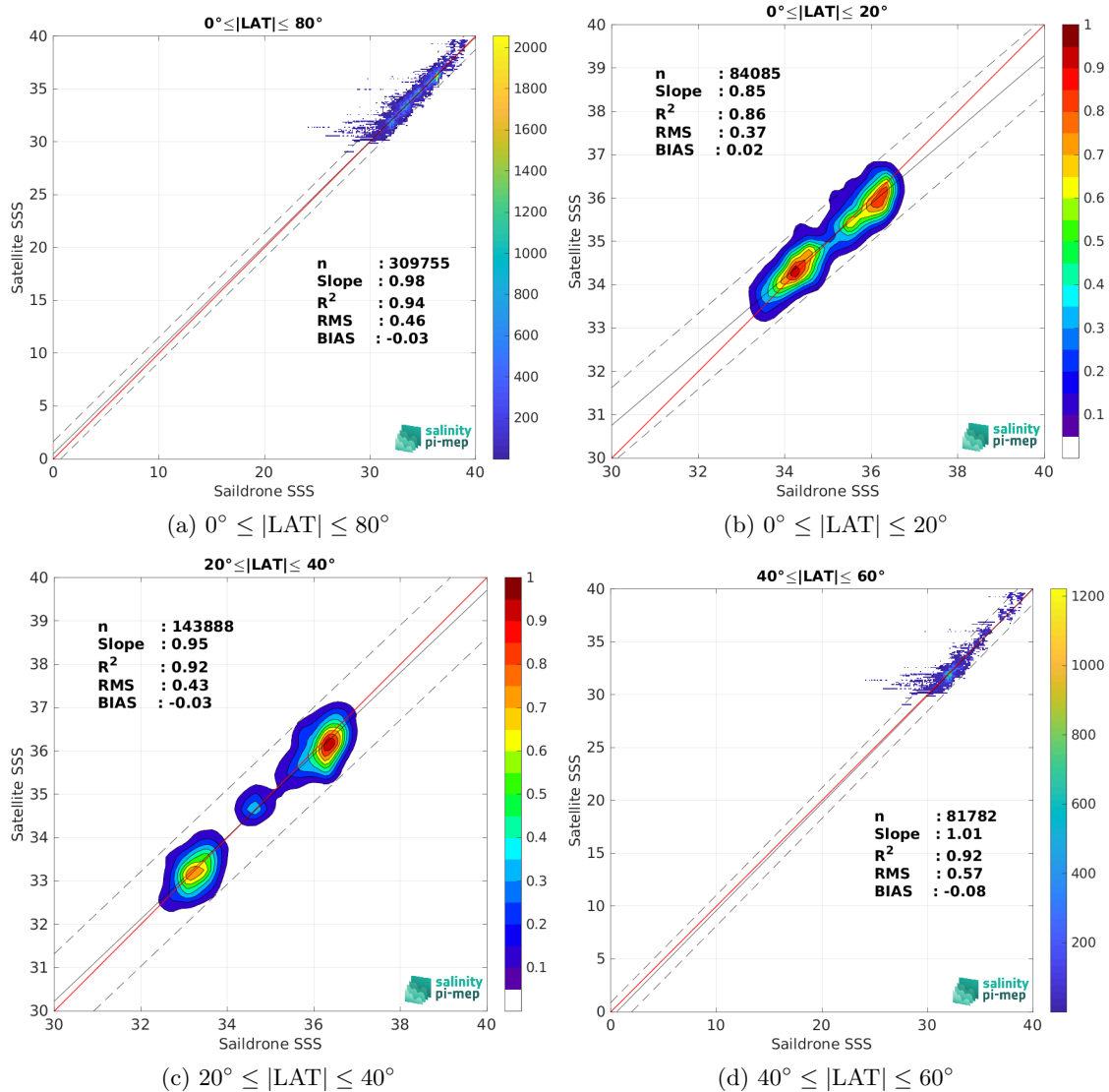
Figure 10: Contour maps of the concentration of SMOS SSS L3 v332 - 9 Days (CATDS-CPDC) SSS (y-axis) versus Saildrone SSS (x-axis) at match-up pairs for different latitude bands. For each plot, the red line shows x=y . The black thin and dashed lines indicate a linear fit through the data cloud and the \pm 95\% confidence levels, respectively. The number match-up pairs n , the slope and R^2 coefficient of the linear fit, the root mean square (RMS) and the mean bias between satellite and in situ data are indicated for each latitude band in each plots.
