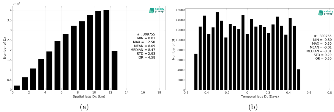
Figure 6: Histograms of the spatial (a) and temporal (b) lags between the location/time of the Saildrone measurement and the date of the corresponding SMOS SSS L3 v332 - 9 Days (CATDS-CPDC) SSS pixel.
