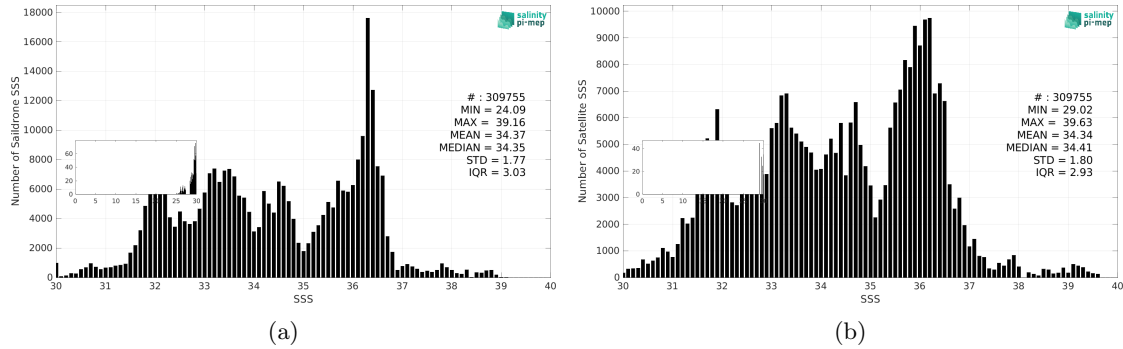
Figure 3: Histograms of SSS from Saildrone (a) and SMOS SSS L3 v332 - 9 Days (CATDS-CPDC) (b) considering all match-up pairs per bins of 0.1 over the SMOS coastal zone (<800km) 60N-60S Pi-MEP region and for the full satellite product period.
