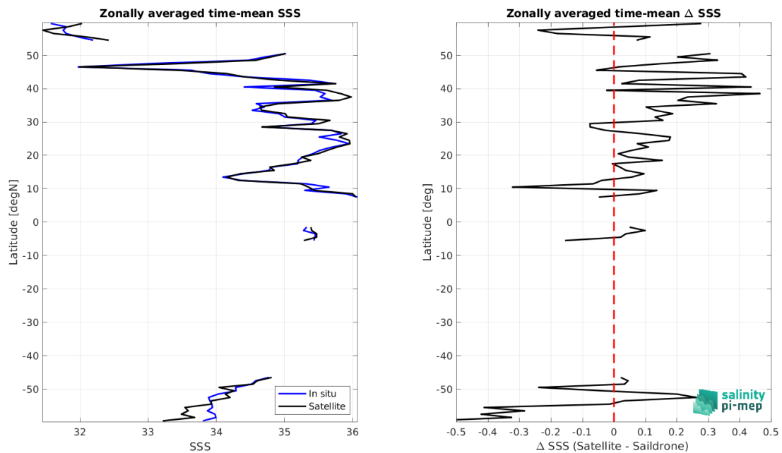
Figure 9: Left panel: Zonal mean SSS from SMOS SSS L3 v332 - 9 Days (CATDS-CPDC) satellite product (black) and from Saildrone (blue). Right panel: Zonal mean of \Delta SSS (Satellite - Saildrone) for all the collected Pi-MEP match-up pairs estimated over the full satellite product period.
