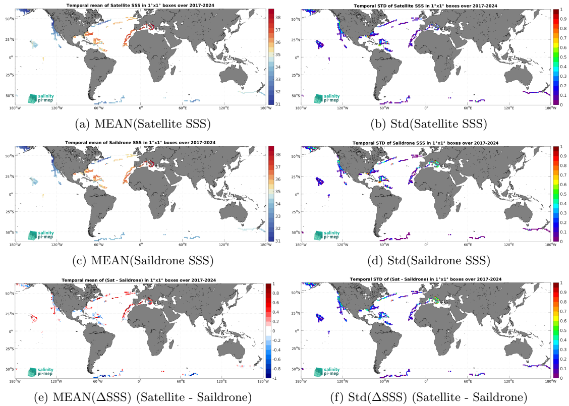
Figure 7: Temporal mean (left) and Std (right) of SSS from SMOS SSS L3 v332 - 9 Days (CATDS-CPDC) (top), Saildrone (middle), and of \Delta SSS (Satellite - Saildrone). Only match-up pairs are used to generate these maps.
