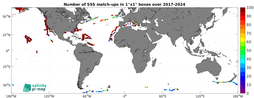
Figure 5: Number of SSS match-ups between Saildrone SSS and the SMOS SSS L3 v332 - 9 Days (CATDS-CPDC) SSS product for the SMOS coastal zone (<800km) 60N-60S Pi-MEP region over 1^\circ \times 1^\circ boxes and for the full satellite product period.
