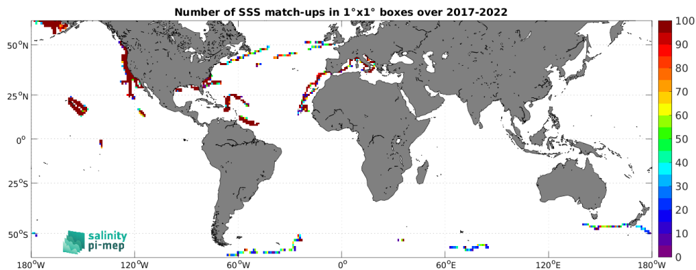
Figure 4: Number of SSS match-ups between Saildrone SSS and the SMOS SSS L3 v332 - 9 Days (CATDS-CPDC) SSS product for the SMOS coastal zone (<800km) 60N-60S Pi-MEP region over 1^\circ \times 1^\circ boxes and for the full satellite product period.
