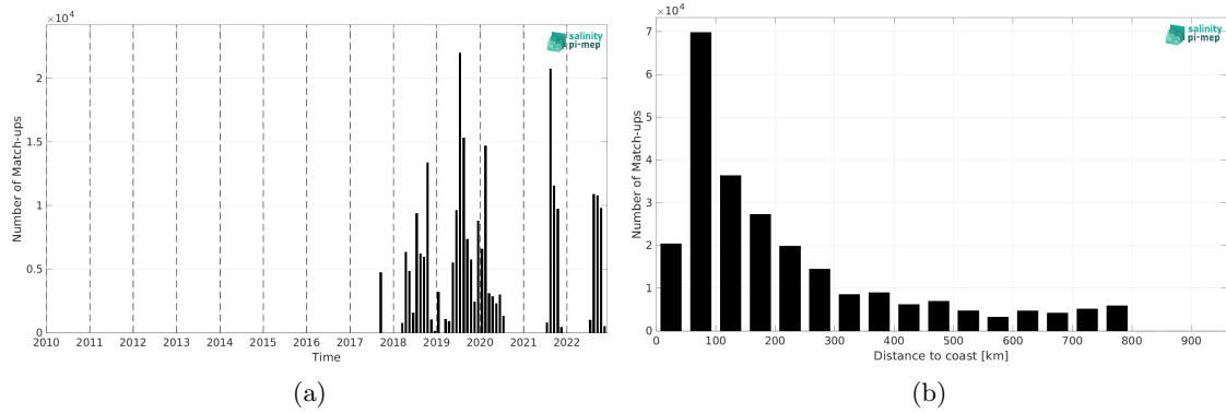
Figure 1: Number of match-ups between Saildrone and SMOS SSS L3 v332 - 9 Days (CATDS-CPDC) SSS as a function of time (a) and as function of the distance to coast (b) over the SMOS coastal zone (<800km) 60N-60S Pi-MEP region and for the full satellite product period.
