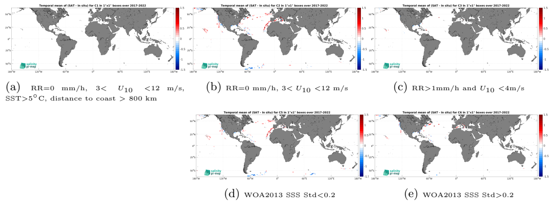
Figure 12: Temporal mean gridded over spatial boxes of size 1^\circ \times 1^\circ of \Delta SSS (SMOS SSS L3 v332 - 9 Days (CATDS-CPDC) - Saildrone) for 5 different subdatasets corresponding to:RR=0 mm/h, 3 < U_{10} < 12 m/s, SST >5^\circ\text{C} , distance to coast > 800 km (a), RR=0 mm/h, 3 < U_{10} < 12 m/s (b), RR >1 mm/h and U_{10} < 4 m/s (c), WOA2013 SSS Std <0.2 (d), WOA2013 SSS Std >0.2 (e).
