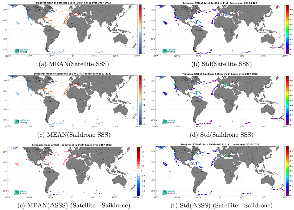
Figure 6: Temporal mean (left) and Std (right) of SSS from SMOS SSS L3 v332 - 9 Days (CATDS-CPDC) (top), Saildrone (middle), and of \Delta SSS (Satellite - Saildrone). Only match-up pairs are used to generate these maps.
