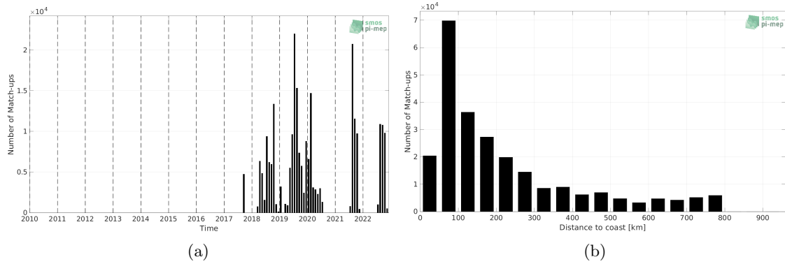
Figure 1: Number of match-ups between Saïdrone and SMOS SSS L3 v332 - 9 Days (CATDS-CPDC) SSS as a function of time (a) and as function of the distance to coast (b) over the SMOS coastal zone (<800km) 60N-60S Pi-MEP region and for the full satellite product period.
