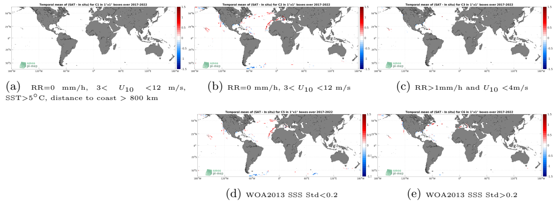
Figure 12: Temporal mean gridded over spatial boxes of size 1^\circ \times 1^\circ of \Delta\text{SSS} (SMOS SSS L3 v332 - 9 Days (CATDS-CPDC) - Sairdrone) for 5 different subdatasets corresponding to:RR=0 mm/h, 3 < U_{10} < 12 m/s, SST >5^\circ\text{C} , distance to coast > 800 km (a), RR=0 mm/h, 3 < U_{10} < 12 m/s (b), RR >1 mm/h and U_{10} < 4 m/s (c), WOA2013 SSS Std <0.2 (d), WOA2013 SSS Std >0.2 (e).
