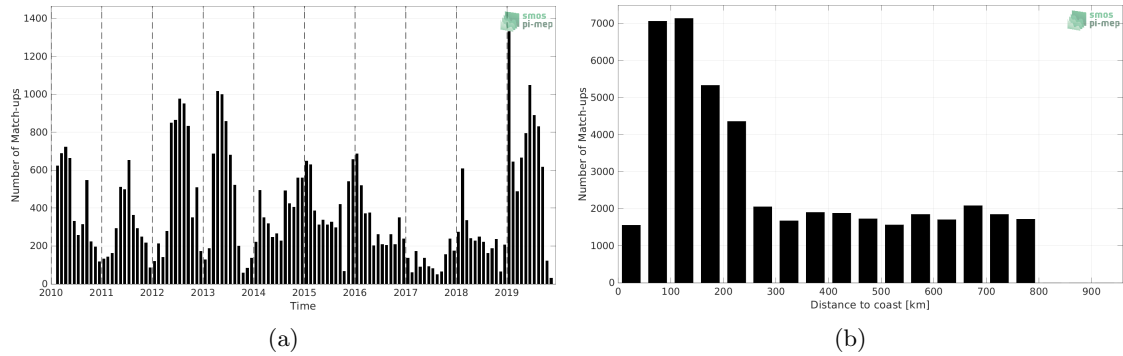
Figure 1: Number of match-ups between Marine mammals and SMOS SSS L3 v332 - 9 Days (CATDS-CPDC) SSS as a function of time (a) and as function of the distance to coast (b) over the SMOS coastal zone (<800km) 60N-60S Pi-MEP region and for the full satellite product period.
