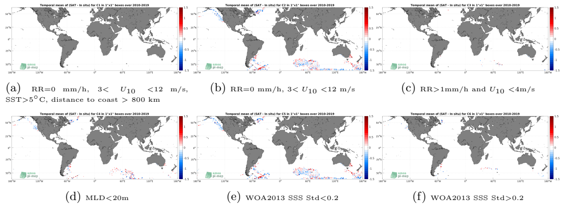
Figure 12: Temporal mean gridded over spatial boxes of size 1^\circ \times 1^\circ of \Delta SSS (SMOS SSS L3 v332 - 9 Days (CATDS-CPDC) - Marine mammals) for 6 different subdatasets corresponding to:RR=0 mm/h, 3 < U_{10} < 12 m/s, SST >5^\circ C, distance to coast > 800 km (a), RR=0 mm/h, 3 < U_{10} < 12 m/s (b), RR >1 mm/h and U_{10} < 4 m/s (c),MLD <20 m (d),WOA2013 SSS Std <0.2 (e),WOA2013 SSS Std >0.2 (f).
