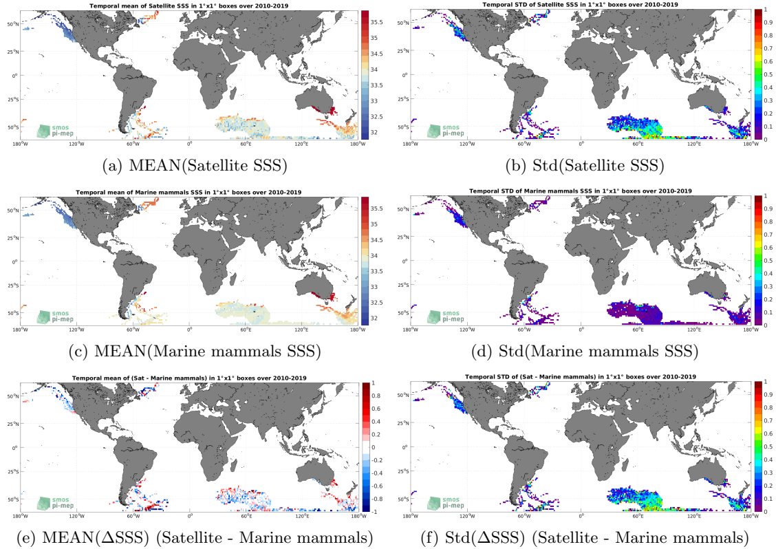
Figure 6: Temporal mean (left) and Std (right) of SSS from SMOS SSS L3 v332 - 9 Days (CATDS-CPDC) (top), Marine mammals (middle), and of \Delta SSS (Satellite - Marine mammals). Only match-up pairs are used to generate these maps.
