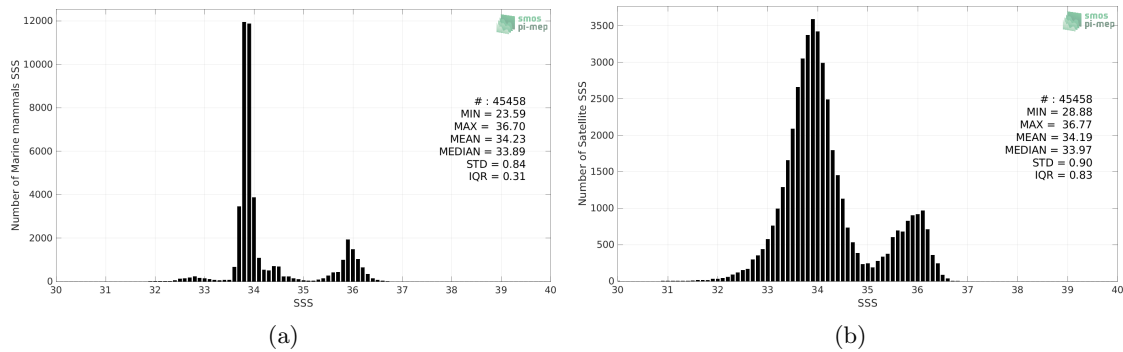
Figure 2: Histograms of SSS from Marine mammals (a) and SMOS SSS L3 v332 - 9 Days (CATDS-CPDC) (b) considering all match-up pairs per bins of 0.1 over the SMOS coastal zone (<800km) 60N-60S Pi-MEP region and for the full satellite product period.
