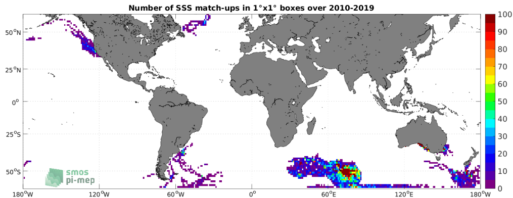
Figure 4: Number of SSS match-ups between Marine mammals SSS and the SMOS SSS L3 v332 - 9 Days (CATDS-CPDC) SSS product for the SMOS coastal zone (<800km) 60N-60S Pi-MEP region over 1^\circ \times 1^\circ boxes and for the full satellite product period.
