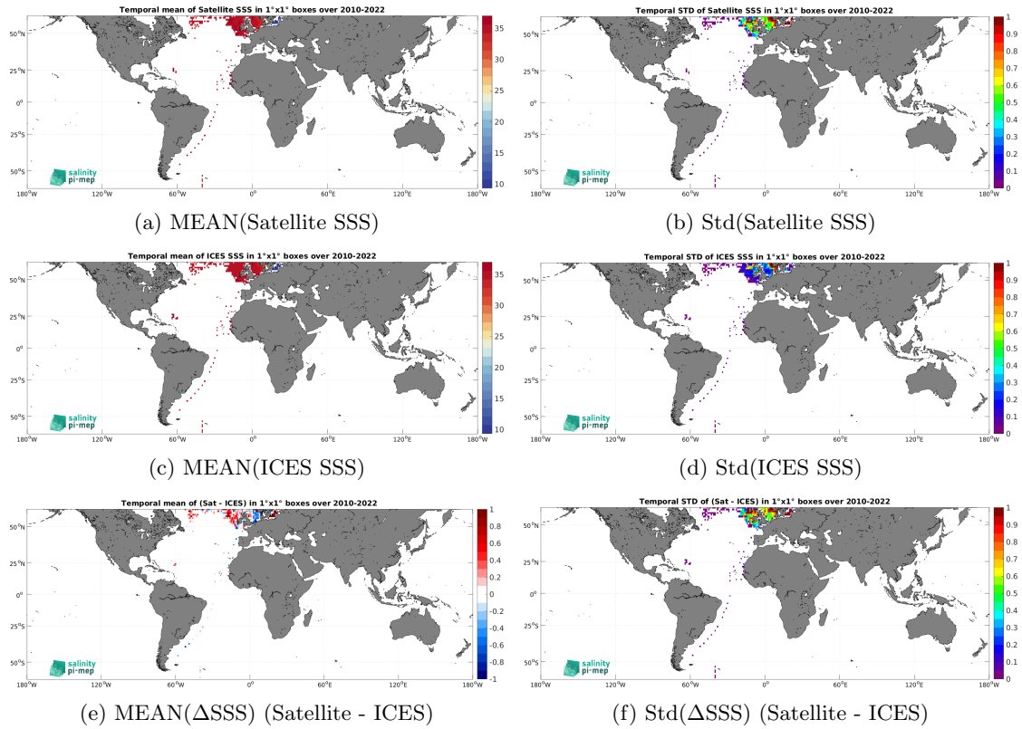
Figure 7: Temporal mean (left) and Std (right) of SSS from SMOS SSS L3 v332 - 9 Days (CATDS-CPDC) (top), ICES (middle), and of \Delta SSS (Satellite - ICES). Only match-up pairs are used to generate these maps.
