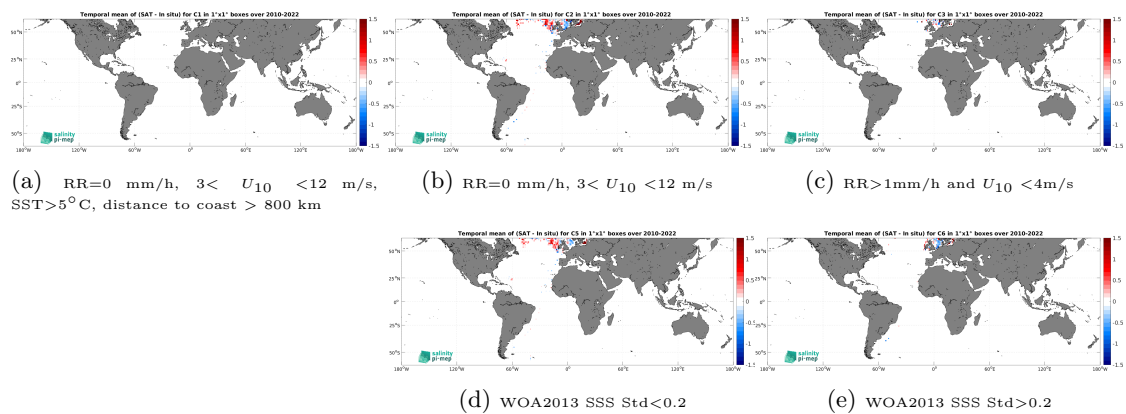
Figure 14: Temporal mean gridded over spatial boxes of size 1^\circ \times 1^\circ of \Delta\text{SSS} (SMOS SSS L3 v332 - 9 Days (CATDS-CPDC) - ICES) for 5 different subdatasets corresponding to:RR=0 mm/h, 3 < U_{10} < 12 m/s, SST >5^\circ\text{C} , distance to coast > 800 km (a), RR=0 mm/h, 3 < U_{10} < 12 m/s (b), RR >1 mm/h and U_{10} < 4 m/s (c), WOA2013 SSS Std <0.2 (d), WOA2013 SSS Std >0.2 (e).
