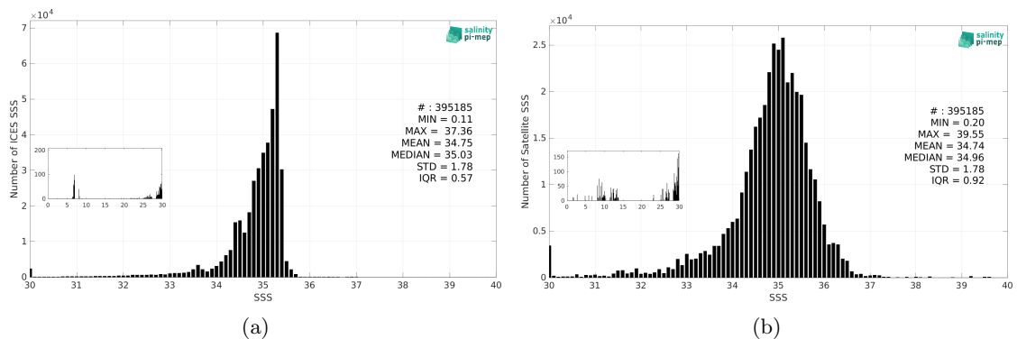
Figure 3: Histograms of SSS from ICES (a) and SMOS SSS L3 v332 - 9 Days (CATDS-CPDC) (b) considering all match-up pairs per bins of 0.1 over the SMOS coastal zone (<800km) 60N-60S Pi-MEP region and for the full satellite product period.
