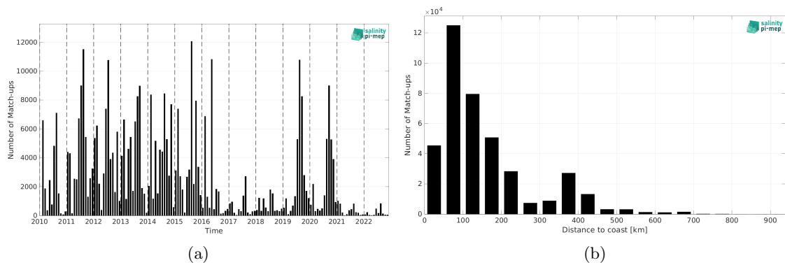
Figure 2: Number of match-ups between ICES and SMOS SSS L3 v332 - 9 Days (CATDS-CPDC) SSS as a function of time (a) and as function of the distance to coast (b) over the SMOS coastal zone (<800km) 60N-60S Pi-MEP region and for the full satellite product period.
