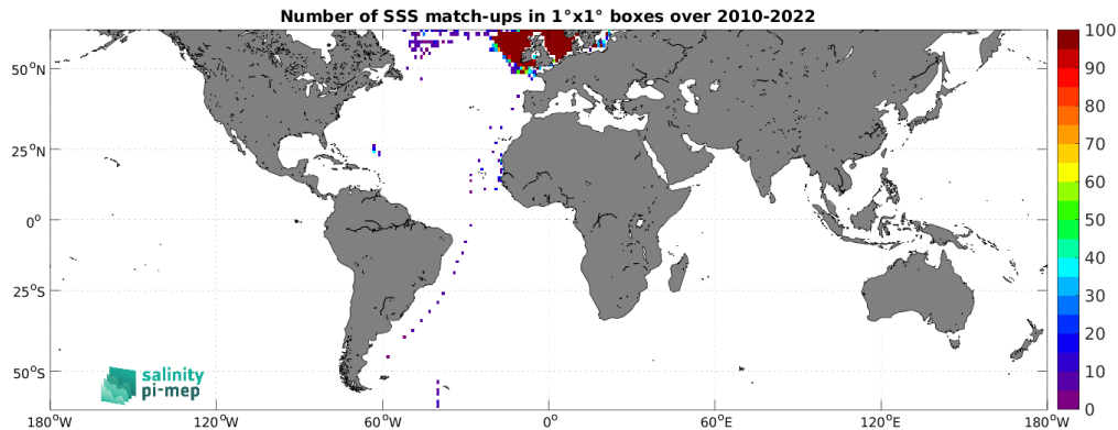
Figure 5: Number of SSS match-ups between ICES SSS and the SMOS SSS L3 v332 - 9 Days (CATDS-CPDC) SSS product for the SMOS coastal zone ( <800\text{km} ) 60N-60S Pi-MEP region over 1^\circ \times 1^\circ boxes and for the full satellite product period.
