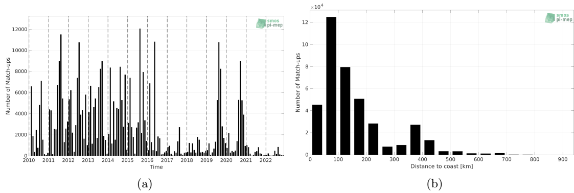
Figure 1: Number of match-ups between ICES and SMOS SSS L3 v332 - 9 Days (CATDS-CPDC) SSS as a function of time (a) and as function of the distance to coast (b) over the SMOS coastal zone ( <800\text{km} ) 60N-60S Pi-MEP region and for the full satellite product period.
