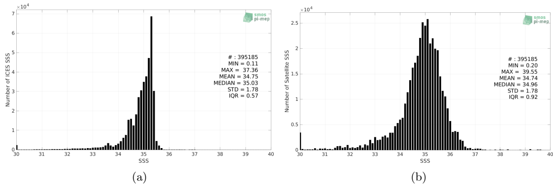
Figure 2: Histograms of SSS from ICES (a) and SMOS SSS L3 v332 - 9 Days (CATDS-CPDC) (b) considering all match-up pairs per bins of 0.1 over the SMOS coastal zone ( <800\text{km} ) 60N-60S Pi-MEP region and for the full satellite product period.
