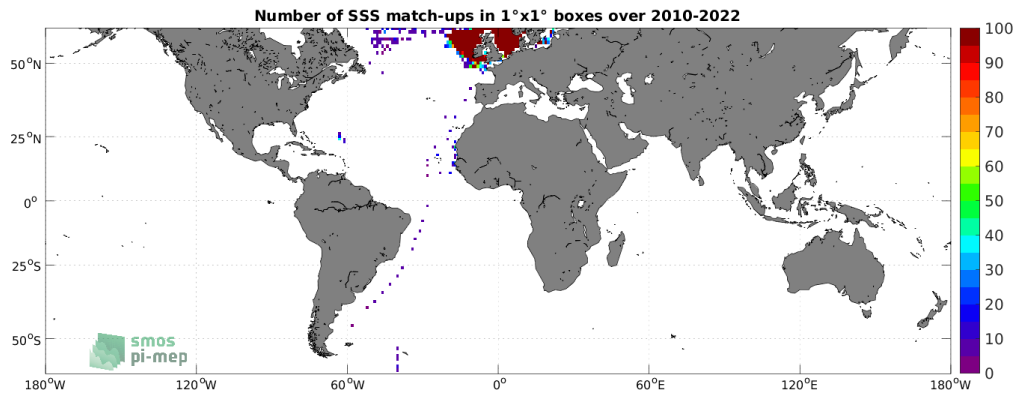
Figure 4: Number of SSS match-ups between ICES SSS and the SMOS SSS L3 v332 - 9 Days (CATDS-CPDC) SSS product for the SMOS coastal zone (<800km) 60N-60S Pi-MEP region over 1^\circ \times 1^\circ boxes and for the full satellite product period.
