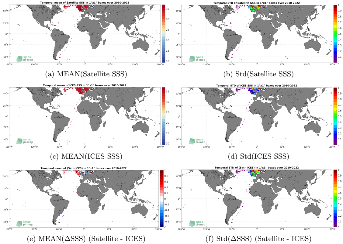
Figure 6: Temporal mean (left) and Std (right) of SSS from SMOS SSS L3 v332 - 9 Days (CATDS-CPDC) (top), ICES (middle), and of \Delta SSS (Satellite - ICES). Only match-up pairs are used to generate these maps.
