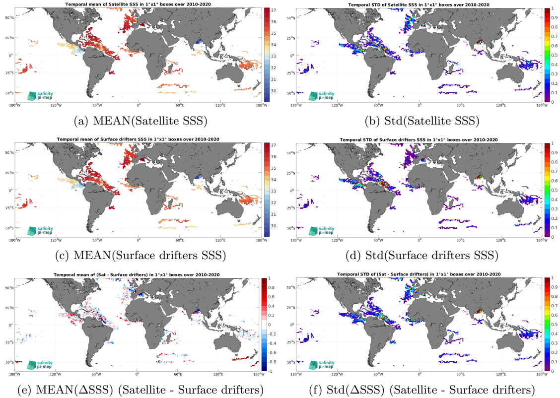
Figure 6: Temporal mean (left) and Std (right) of SSS from SMOS SSS L3 v332 - 9 Days (CATDS-CPDC) (top), Surface drifters (middle), and of \Delta SSS (Satellite - Surface drifters). Only match-up pairs are used to generate these maps.
