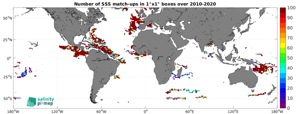
Figure 4: Number of SSS match-ups between Surface drifters SSS and the SMOS SSS L3 v332 - 9 Days (CATDS-CPDC) SSS product for the SMOS coastal zone ( <800\text{km} ) 60N-60S Pi-MEP region over 1^\circ \times 1^\circ boxes and for the full satellite product period.
