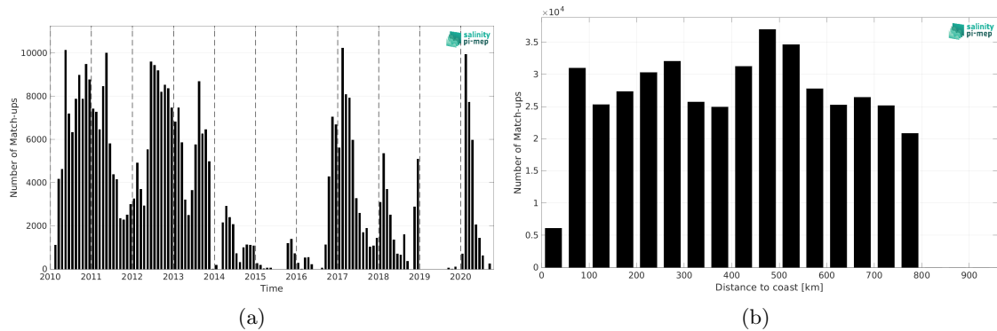
Figure 2: Number of match-ups between Surface drifters and SMOS SSS L3 v332 - 9 Days (CATDS-CPDC) SSS as a function of time (a) and as function of the distance to coast (b) over the SMOS coastal zone (<800km) 60N-60S Pi-MEP region and for the full satellite product period.
