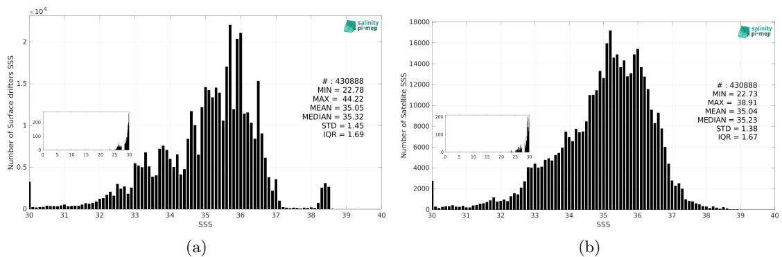
Figure 3: Histograms of SSS from Surface drifters (a) and SMOS SSS L3 v332 - 9 Days (CATDS-CPDC) (b) considering all match-up pairs per bins of 0.1 over the SMOS coastal zone (<800km) 60N-60S Pi-MEP region and for the full satellite product period.
