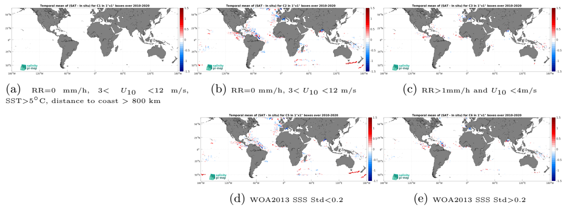
Figure 13: Temporal mean gridded over spatial boxes of size 1^\circ \times 1^\circ of \Delta SSS (SMOS SSS L3 v332 - 9 Days (CATDS-CPDC) - Surface drifters) for 5 different subdatasets corresponding to:RR=0 mm/h, 3 < U_{10} < 12 m/s, SST >5^\circ C, distance to coast > 800 km (a), RR=0 mm/h, 3 < U_{10} < 12 m/s (b), RR >1 mm/h and U_{10} < 4 m/s (c), WOA2013 SSS Std <0.2 (d), WOA2013 SSS Std >0.2 (e).
