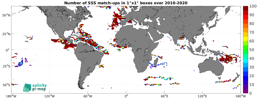
Figure 4: Number of SSS match-ups between Surface drifters SSS and the SMOS SSS L3 v332 - 9 Days (CATDS-CPDC) SSS product for the SMOS coastal zone (<800km) 60N-60S Pi-MEP region over 1^{\circ} \times 1^{\circ} boxes and for the full satellite product period.
