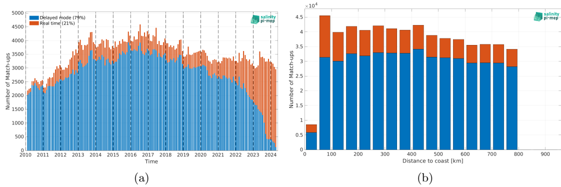
Figure 2: Number of match-ups between Argo and SMOS SSS L3 v332 - 9 Days (CATDS-CPDC) SSS as a function of time (a) and as function of the distance to coast (b) over the SMOS coastal zone (<800km) 60N-60S Pi-MEP region and for the full satellite product period.
