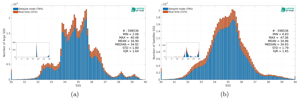
Figure 3: Histograms of SSS from Argo (a) and SMOS SSS L3 v332 - 9 Days (CATDS-CPDC) (b) considering all match-up pairs per bins of 0.1 over the SMOS coastal zone (<800km) 60N-60S Pi-MEP region and for the full satellite product period.
