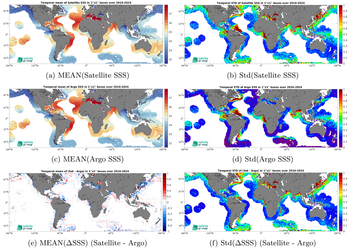
Figure 7: Temporal mean (left) and Std (right) of SSS from SMOS SSS L3 v332 - 9 Days (CATDS-CPDC) (top), Argo (middle), and of \Delta SSS (Satellite - Argo). Only match-up pairs are used to generate these maps.
