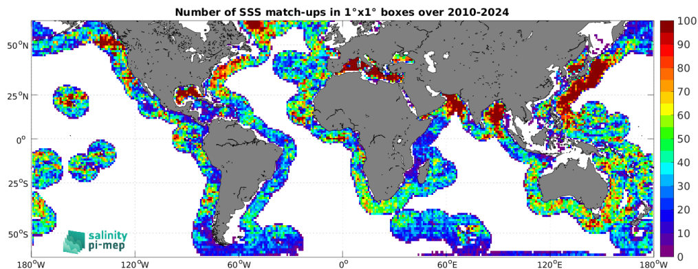
Figure 5: Number of SSS match-ups between Argo SSS and the SMOS SSS L3 v332 - 9 Days (CATDS-CPDC) SSS product for the SMOS coastal zone ( <800\text{km} ) 60N-60S Pi-MEP region over 1^\circ \times 1^\circ boxes and for the full satellite product period.
