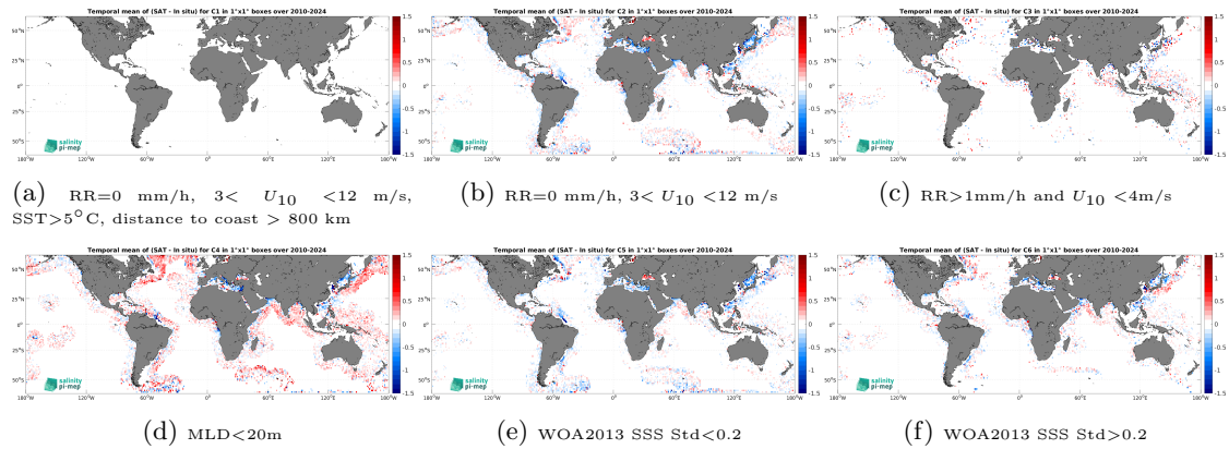
Figure 14: Temporal mean gridded over spatial boxes of size 1^\circ \times 1^\circ of \Delta SSS (SMOS SSS L3 v332 - 9 Days (CATDS-CPDC) - Argo) for 6 different subdatasets corresponding to:RR=0 mm/h, 3 < U_{10} < 12 m/s, SST >5^\circ C, distance to coast > 800 km (a), RR=0 mm/h, 3 < U_{10} < 12 m/s (b), RR >1 mm/h and U_{10} < 4 m/s (c),MLD <20 m (d),WOA2013 SSS Std <0.2 (e),WOA2013 SSS Std >0.2 (f).
