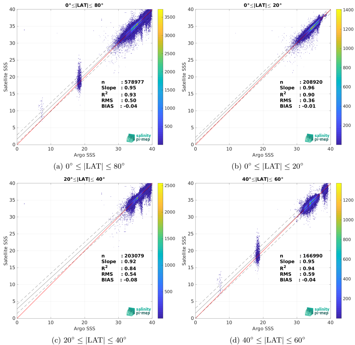
Figure 9: Contour maps of the concentration of SMOS SSS L3 v332 - 9 Days (CATDS-CPDC) SSS (y-axis) versus Argo SSS (x-axis) at match-up pairs for different latitude bands. For each plot, the red line shows x=y . The black thin and dashed lines indicate a linear fit through the data cloud and the \pm 95\% confidence levels, respectively. The number match-up pairs n , the slope and R^2 coefficient of the linear fit, the root mean square (RMS) and the mean bias between satellite and in situ data are indicated for each latitude band in each plot.
