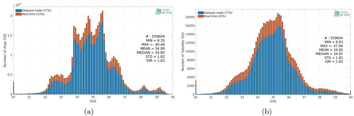
Figure 2: Histograms of SSS from Argo (a) and SMOS SSS L3 v332 - 9 Days (CATDS-CPDC) (b) considering all match-up pairs per bins of 0.1 over the SMOS coastal zone (<800km) 60N-60S Pi-MEP region and for the full satellite product period.
