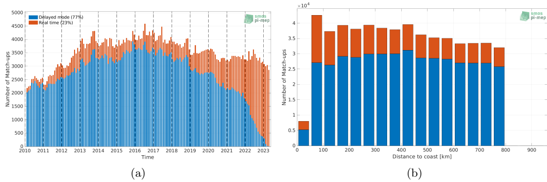
Figure 1: Number of match-ups between Argo and SMOS SSS L3 v332 - 9 Days (CATDS-CPDC) SSS as a function of time (a) and as function of the distance to coast (b) over the SMOS coastal zone (<800km) 60N-60S Pi-MEP region and for the full satellite product period.
