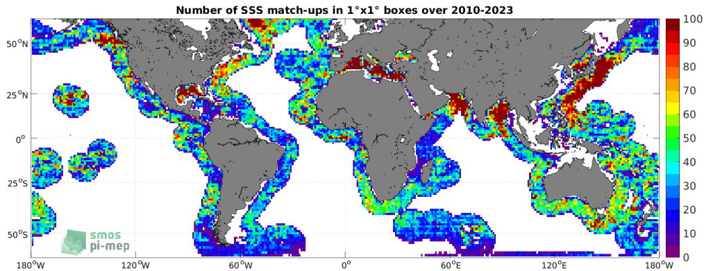
Figure 4: Number of SSS match-ups between Argo SSS and the SMOS SSS L3 v332 - 9 Days (CATDS-CPDC) SSS product for the SMOS coastal zone (<800km) 60N-60S Pi-MEP region over 1^\circ \times 1^\circ boxes and for the full satellite product period.
