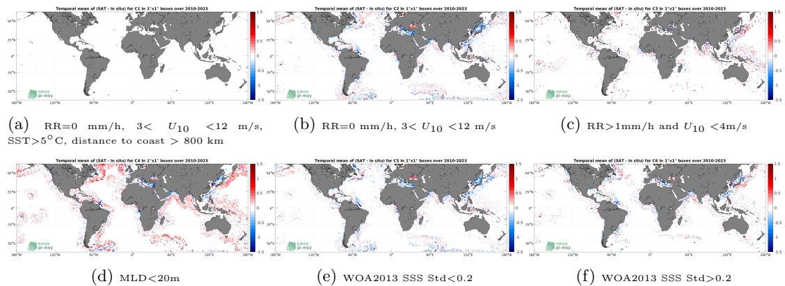
Figure 12: Temporal mean gridded over spatial boxes of size 1^\circ \times 1^\circ of \Delta SSS (SMOS SSS L3 v332 - 9 Days (CATDS-CPDC) - Argo) for 6 different subdatasets corresponding to:RR=0 mm/h, 3 < U_{10} < 12 m/s, SST >5^\circ C, distance to coast > 800 km (a), RR=0 mm/h, 3 < U_{10} < 12 m/s (b), RR >1 mm/h and U_{10} < 4 m/s (c),MLD <20 m (d),WOA2013 SSS Std <0.2 (e),WOA2013 SSS Std >0.2 (f).
