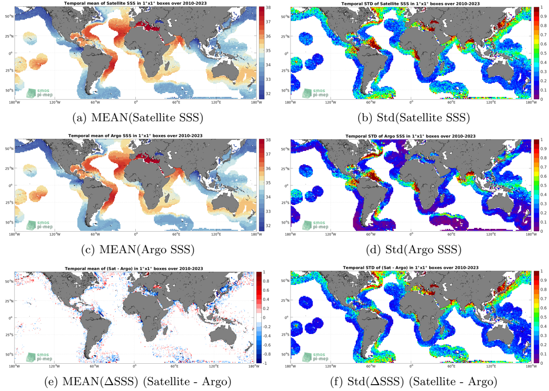
Figure 6: Temporal mean (left) and Std (right) of SSS from SMOS SSS L3 v332 - 9 Days (CATDS-CPDC) (top), Argo (middle), and of \Delta SSS (Satellite - Argo). Only match-up pairs are used to generate these maps.
