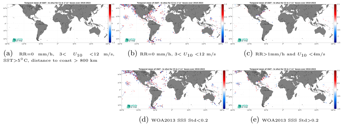
Figure 12: Temporal mean gridded over spatial boxes of size 1^\circ \times 1^\circ of \Delta\text{SSS} (SMOS SSS L2Q v331 - 0.25 Deg (CATDS-CPDC) - TSG (SAMOS)) for 5 different subdatasets corresponding to:RR=0 mm/h, 3 < U_{10} < 12 m/s, SST >5^\circ\text{C} , distance to coast > 800 km (a), RR=0 mm/h, 3 < U_{10} < 12 m/s (b), RR >1 mm/h and U_{10} < 4 m/s (c), WOA2013 SSS Std <0.2 (d), WOA2013 SSS Std >0.2 (e).
