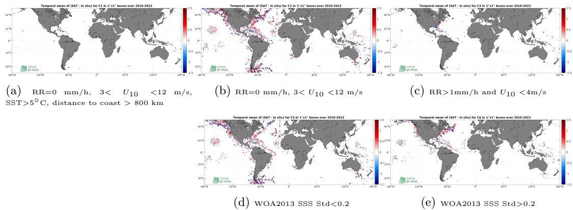
Figure 12: Temporal mean gridded over spatial boxes of size 1^\circ \times 1^\circ of \Delta SSS (SMOS SSS L2Q v331 - 0.25 Deg (CATDS-CPDC) - TSG (SAMOS)) for 5 different subdatasets corresponding to:RR=0 mm/h, 3 < U_{10} < 12 m/s, SST >5^\circ C, distance to coast > 800 km (a), RR=0 mm/h, 3 < U_{10} < 12 m/s (b), RR >1 mm/h and U_{10} < 4 m/s (c), WOA2013 SSS Std <0.2 (d), WOA2013 SSS Std >0.2 (e).
