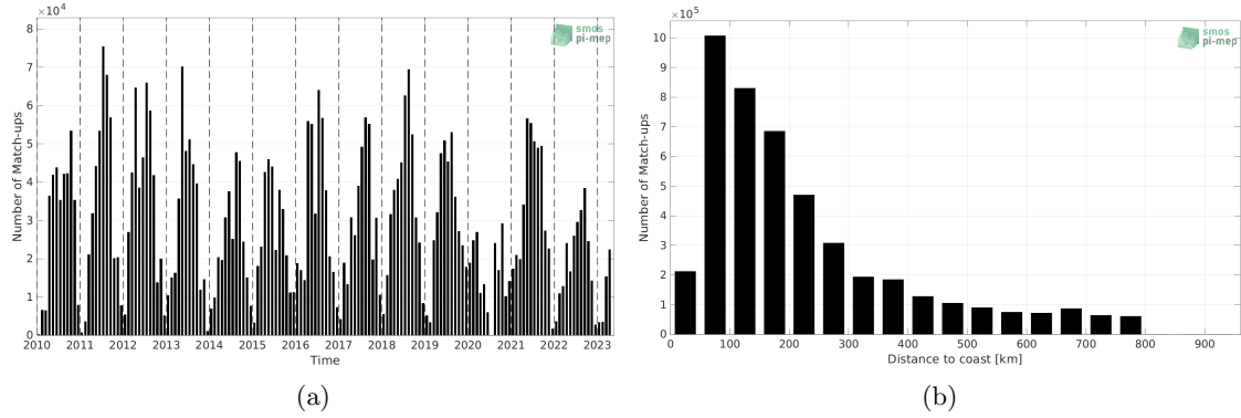
Figure 1: Number of match-ups between TSG (SAMOS) and SMOS SSS L2Q v331 - 0.25 Deg (CATDS-CPDC) SSS as a function of time (a) and as function of the distance to coast (b) over the SMOS coastal zone (<800km) 60N-60S Pi-MEP region and for the full satellite product period.
