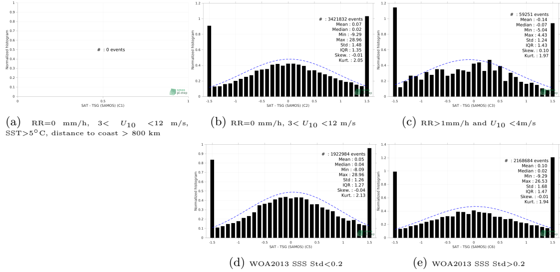
Figure 13: Normalized histogram of \Delta SSS (SMOS SSS L2Q v331 - 0.25 Deg (CATDS-CPDC) - TSG (SAMOS)) for 5 different subdatasets corresponding to: RR=0 mm/h, 3 < U_{10} < 12 m/s, SST>5°C, distance to coast > 800 km (a), RR=0 mm/h, 3 < U_{10} < 12 m/s (b), RR>1mm/h and U_{10} < 4 m/s (c), WOA2013 SSS Std<0.2 (d), WOA2013 SSS Std>0.2 (e).
