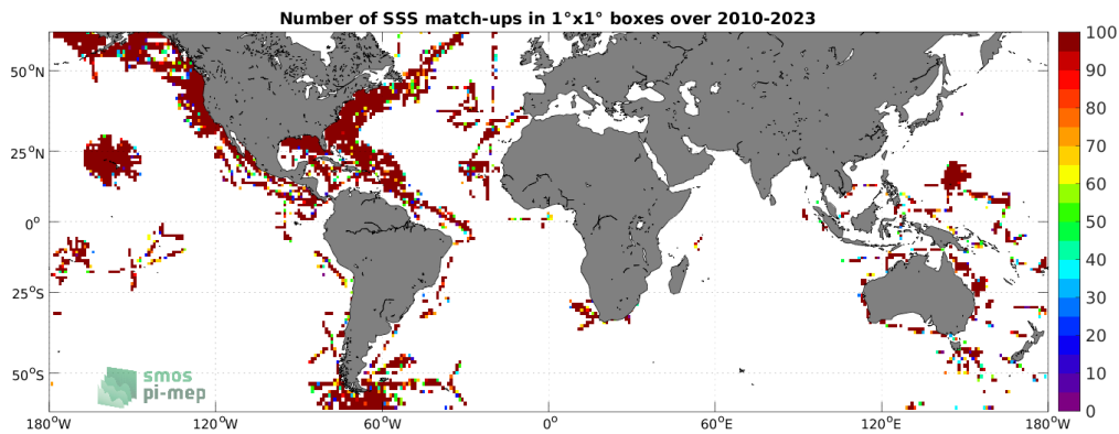
Figure 4: Number of SSS match-ups between TSG (SAMOS) SSS and the SMOS SSS L2Q v331 - 0.25 Deg (CATDS-CPDC) SSS product for the SMOS coastal zone (<800km) 60N-60S Pi-MEP region over 1^\circ \times 1^\circ boxes and for the full satellite product period.
