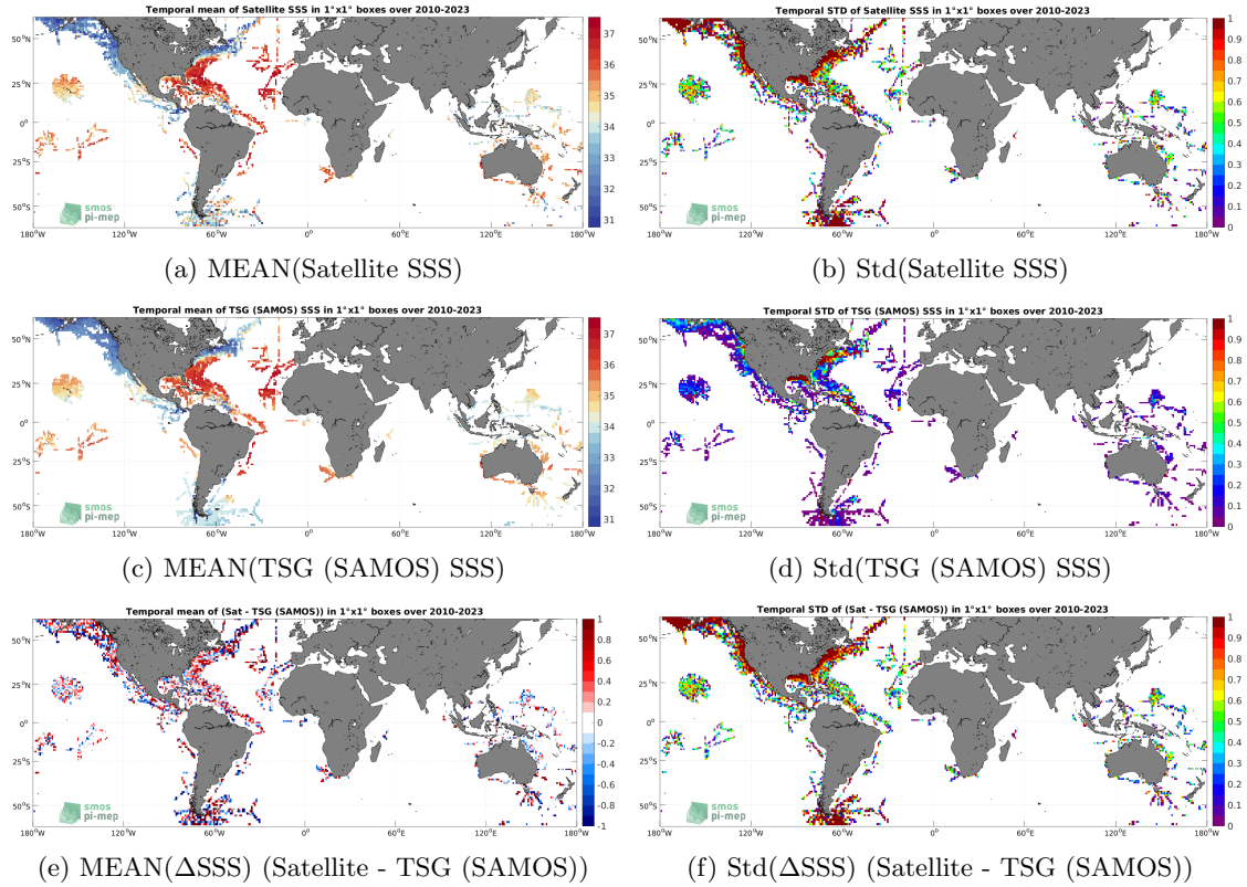
Figure 6: Temporal mean (left) and Std (right) of SSS from SMOS SSS L2Q v331 - 0.25 Deg (CATDS-CPDC) (top), TSG (SAMOS) (middle), and of \Delta SSS (Satellite - TSG (SAMOS)). Only match-up pairs are used to generate these maps.
