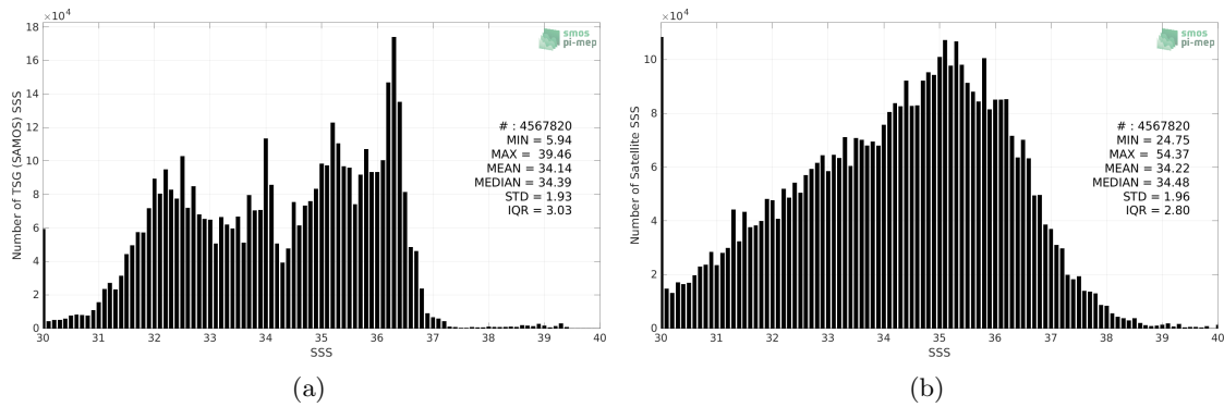
Figure 2: Histograms of SSS from TSG (SAMOS) (a) and SMOS SSS L2Q v331 - 0.25 Deg (CATDS-CPDC) (b) considering all match-up pairs per bins of 0.1 over the SMOS coastal zone (<800km) 60N-60S Pi-MEP region and for the full satellite product period.
