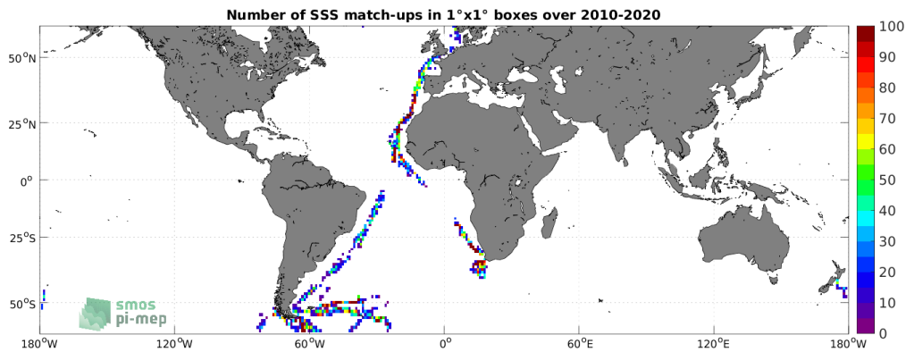
Figure 4: Number of SSS match-ups between TSG (Polarstern) SSS and the SMOS SSS L2Q v331 - 0.25 Deg (CATDS-CPDC) SSS product for the SMOS coastal zone (<800km) 60N-60S Pi-MEP region over 1^\circ \times 1^\circ boxes and for the full satellite product period.
