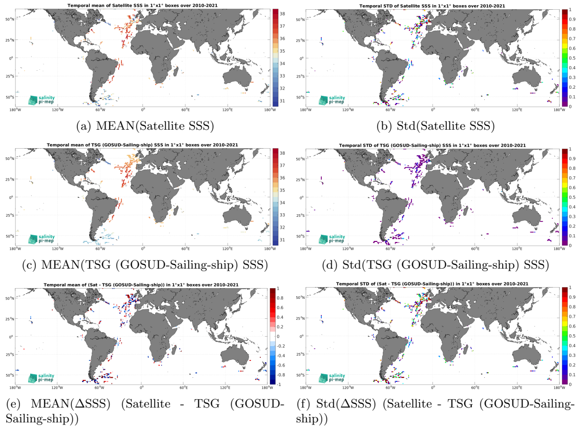
Figure 6: Temporal mean (left) and Std (right) of SSS from SMOS SSS L2Q v331 - 0.25 Deg (CATDS-CPDC) (top), TSG (GOSUD-Sailing-ship) (middle), and of \Delta SSS (Satellite - TSG (GOSUD-Sailing-ship)). Only match-up pairs are used to generate these maps.
