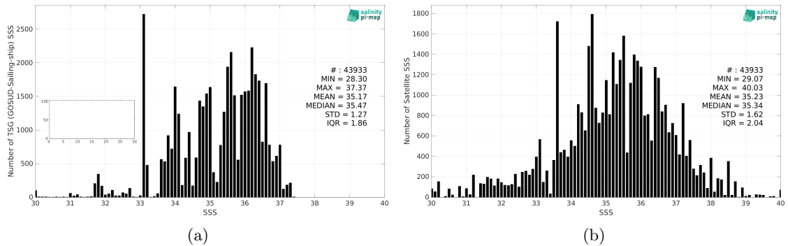
Figure 2: Histograms of SSS from TSG (GOSUD-Sailing-ship) (a) and SMOS SSS L2Q v331 - 0.25 Deg (CATDS-CPDC) (b) considering all match-up pairs per bins of 0.1 over the SMOS coastal zone (<800km) 60N-60S Pi-MEP region and for the full satellite product period.
