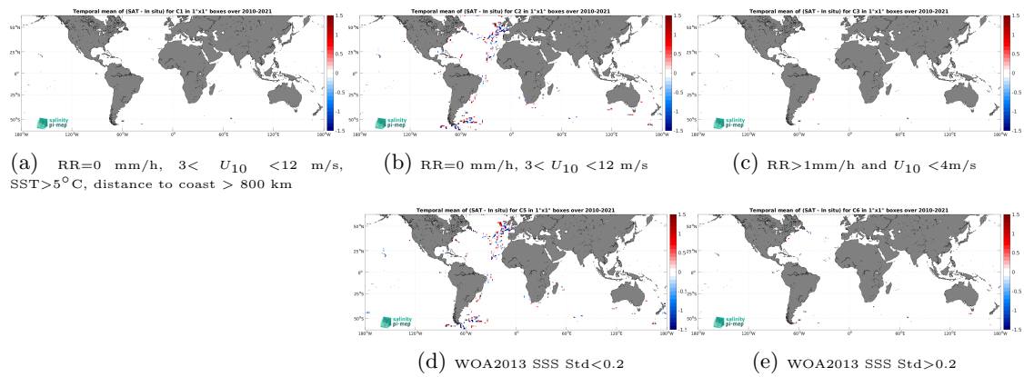
Figure 12: Temporal mean gridded over spatial boxes of size 1^\circ \times 1^\circ of \Delta\text{SSS} (SMOS SSS L2Q v331 - 0.25 Deg (CATDS-CPDC) - TSG (GOSUD-Sailing-ship)) for 5 different subdatasets corresponding to: RR=0 mm/h, 3 < U_{10} < 12 m/s, SST >5^\circ\text{C} , distance to coast > 800 km (a), RR=0 mm/h, 3 < U_{10} < 12 m/s (b), RR >1 mm/h and U_{10} < 4 m/s (c), WOA2013 SSS Std <0.2 (d), WOA2013 SSS Std >0.2 (e).
