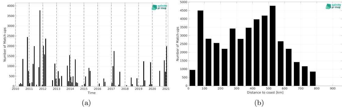
Figure 1: Number of match-ups between TSG (GOSUD-Sailing-ship) and SMOS SSS L2Q v331 - 0.25 Deg (CATDS-CPDC) SSS as a function of time (a) and as function of the distance to coast (b) over the SMOS coastal zone (<800km) 60N-60S Pi-MEP region and for the full satellite product period.
