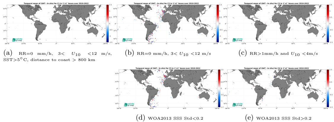
Figure 12: Temporal mean gridded over spatial boxes of size 1^\circ \times 1^\circ of \Delta\text{SSS} (SMOS SSS L2Q v331 - 0.25 Deg (CATDS-CPDC) - TSG (CSIC-UTM)) for 5 different subdatasets corresponding to:RR=0 mm/h, 3 < U_{10} < 12 m/s, SST >5^\circ\text{C} , distance to coast > 800 km (a), RR=0 mm/h, 3 < U_{10} < 12 m/s (b), RR >1 mm/h and U_{10} < 4 m/s (c), WOA2013 SSS Std <0.2 (d), WOA2013 SSS Std >0.2 (e).
