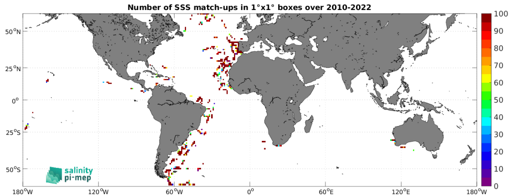
Figure 4: Number of SSS match-ups between TSG (CSIC-UTM) SSS and the SMOS SSS L2Q v331 - 0.25 Deg (CATDS-CPDC) SSS product for the SMOS coastal zone (<800km) 60N-60S Pi-MEP region over 1^\circ \times 1^\circ boxes and for the full satellite product period.
