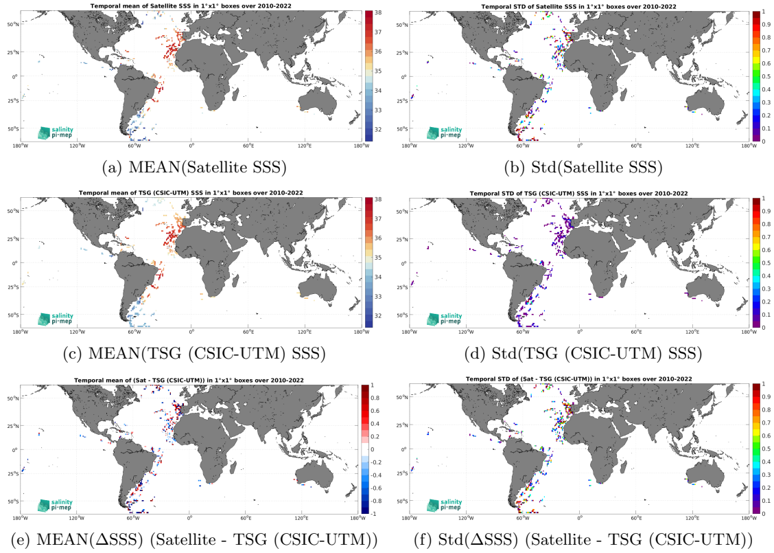
Figure 6: Temporal mean (left) and Std (right) of SSS from SMOS SSS L2Q v331 - 0.25 Deg (CATDS-CPDC) (top), TSG (CSIC-UTM) (middle), and of \Delta SSS (Satellite - TSG (CSIC-UTM)). Only match-up pairs are used to generate these maps.
