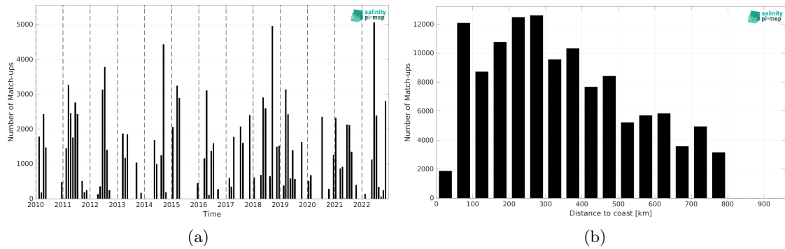
Figure 1: Number of match-ups between TSG (CSIC-UTM) and SMOS SSS L2Q v331 - 0.25 Deg (CATDS-CPDC) SSS as a function of time (a) and as function of the distance to coast (b) over the SMOS coastal zone (<800km) 60N-60S Pi-MEP region and for the full satellite product period.
