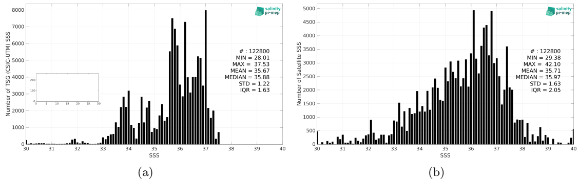
Figure 2: Histograms of SSS from TSG (CSIC-UTM) (a) and SMOS SSS L2Q v331 - 0.25 Deg (CATDS-CPDC) (b) considering all match-up pairs per bins of 0.1 over the SMOS coastal zone (<800km) 60N-60S Pi-MEP region and for the full satellite product period.
