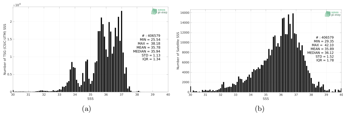
Figure 2: Histograms of SSS from TSG (CSIC-UTM) (a) and SMOS SSS L2Q v331 - 0.25 Deg (CATDS-CPDC) (b) considering all match-up pairs per bins of 0.1 over the SMOS coastal zone (<800km) 60N-60S Pi-MEP region and for the full satellite product period.
