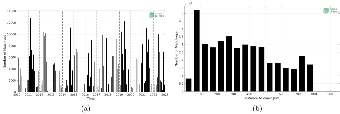
Figure 1: Number of match-ups between TSG (CSIC-UTM) and SMOS SSS L2Q v331 - 0.25 Deg (CATDS-CPDC) SSS as a function of time (a) and as function of the distance to coast (b) over the SMOS coastal zone (<800km) 60N-60S Pi-MEP region and for the full satellite product period.
