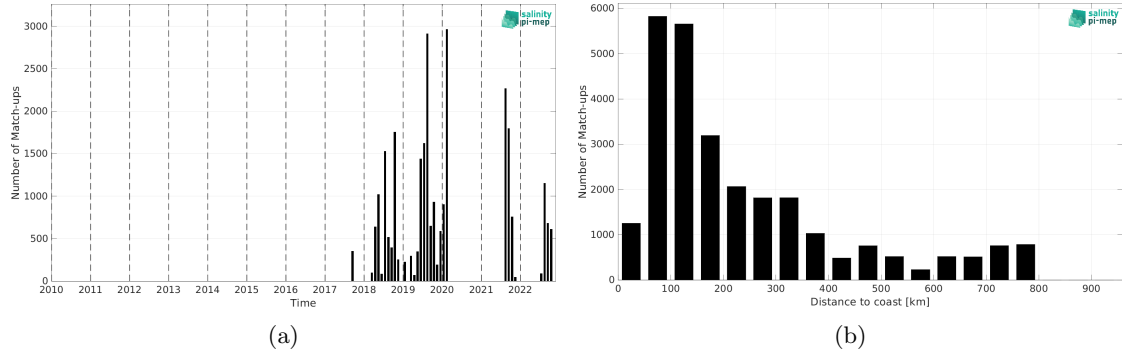
Figure 1: Number of match-ups between Saildrone and SMOS SSS L2Q v331 - 0.25 Deg (CATDS-CPDC) SSS as a function of time (a) and as function of the distance to coast (b) over the SMOS coastal zone (<800km) 60N-60S Pi-MEP region and for the full satellite product period.
