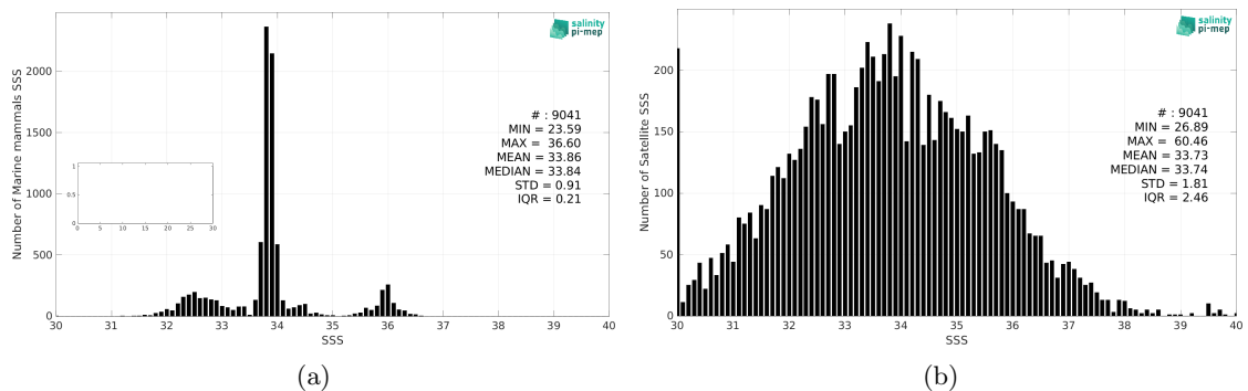
Figure 2: Histograms of SSS from Marine mammals (a) and SMOS SSS L2Q v331 - 0.25 Deg (CATDS-CPDC) (b) considering all match-up pairs per bins of 0.1 over the SMOS coastal zone (<800km) 60N-60S Pi-MEP region and for the full satellite product period.
