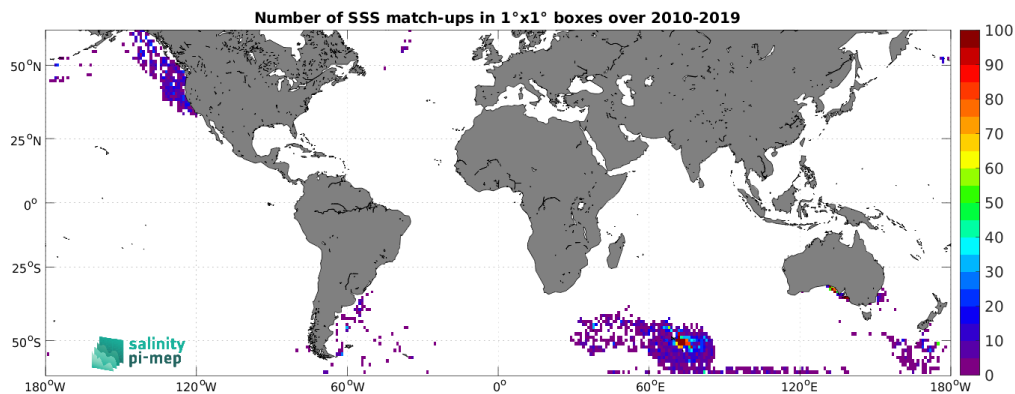
Figure 4: Number of SSS match-ups between Marine mammals SSS and the SMOS SSS L2Q v331 - 0.25 Deg (CATDS-CPDC) SSS product for the SMOS coastal zone (<800km) 60N-60S Pi-MEP region over 1^\circ \times 1^\circ boxes and for the full satellite product period.
