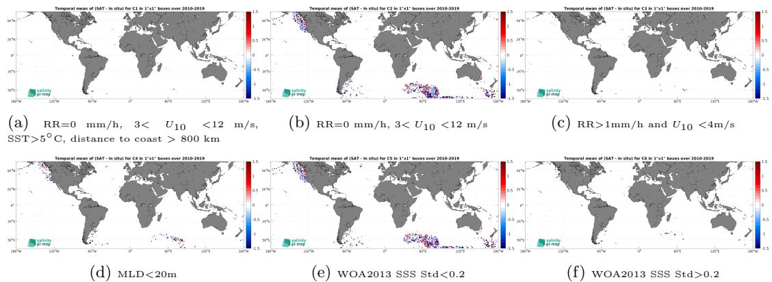
Figure 12: Temporal mean gridded over spatial boxes of size 1^\circ \times 1^\circ of \Delta SSS (SMOS SSS L2Q v331 - 0.25 Deg (CATDS-CPDC) - Marine mammals) for 6 different subdatasets corresponding to:RR=0 mm/h, 3 < U_{10} < 12 m/s, SST >5^\circ C, distance to coast > 800 km (a), RR=0 mm/h, 3 < U_{10} < 12 m/s (b), RR >1 mm/h and U_{10} < 4 m/s (c),MLD <20 m (d),WOA2013 SSS Std <0.2 (e),WOA2013 SSS Std >0.2 (f).
