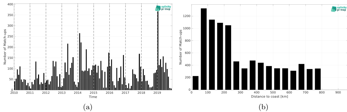
Figure 1: Number of match-ups between Marine mammals and SMOS SSS L2Q v331 - 0.25 Deg (CATDS-CPDC) SSS as a function of time (a) and as function of the distance to coast (b) over the SMOS coastal zone (<800km) 60N-60S Pi-MEP region and for the full satellite product period.
