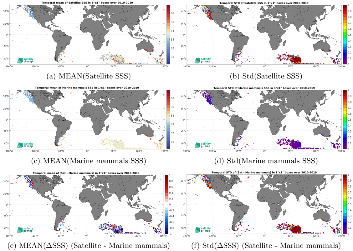
Figure 6: Temporal mean (left) and Std (right) of SSS from SMOS SSS L2Q v331 - 0.25 Deg (CATDS-CPDC) (top), Marine mammals (middle), and of \Delta SSS (Satellite - Marine mammals). Only match-up pairs are used to generate these maps.
