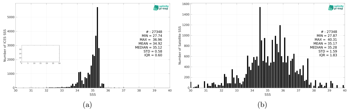
Figure 2: Histograms of SSS from ICES (a) and SMOS SSS L2Q v331 - 0.25 Deg (CATDS-CPDC) (b) considering all match-up pairs per bins of 0.1 over the SMOS coastal zone (<800km) 60N-60S Pi-MEP region and for the full satellite product period.
