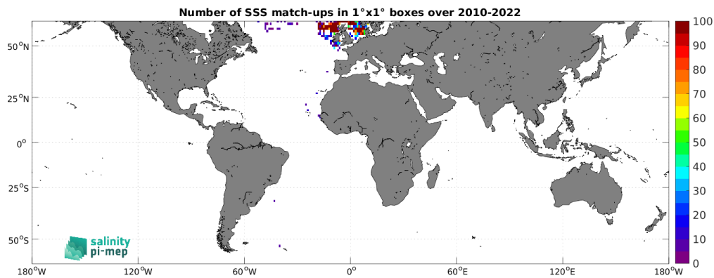
Figure 4: Number of SSS match-ups between ICES SSS and the SMOS SSS L2Q v331 - 0.25 Deg (CATDS-CPDC) SSS product for the SMOS coastal zone (<800km) 60N-60S Pi-MEP region over 1^\circ \times 1^\circ boxes and for the full satellite product period.
