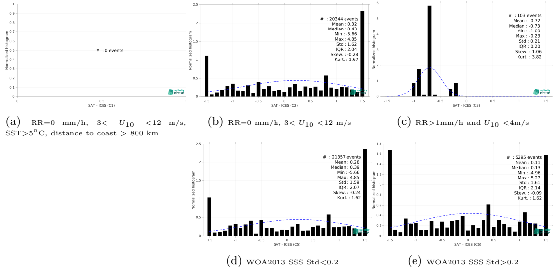
Figure 13: Normalized histogram of \Delta SSS (SMOS SSS L2Q v331 - 0.25 Deg (CATDS-CPDC) - ICES) for 5 different subdatasets corresponding to: RR=0 mm/h, 3 < U_{10} < 12 m/s, SST > 5°C, distance to coast > 800 km (a), RR=0 mm/h, 3 < U_{10} < 12 m/s (b), RR > 1mm/h and U_{10} < 4 m/s (c), WOA2013 SSS Std < 0.2 (d), WOA2013 SSS Std > 0.2 (e).
