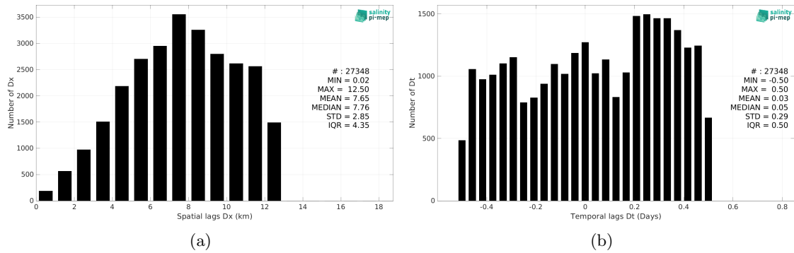
Figure 5: Histograms of the spatial (a) and temporal (b) lags between the location/time of the ICES measurement and the date of the corresponding SMOS SSS L2Q v331 - 0.25 Deg (CATDS-CPDC) SSS pixel.
