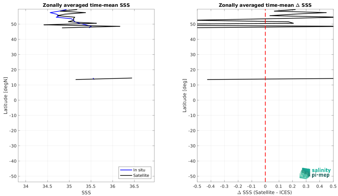
Figure 8: Left panel: Zonal mean SSS from SMOS SSS L2Q v331 - 0.25 Deg (CATDS-CPDC) satellite product (black) and from ICES (blue). Right panel: Zonal mean of \Delta SSS (Satellite - ICES) for all the collected Pi-MEP match-up pairs estimated over the full satellite product period.
