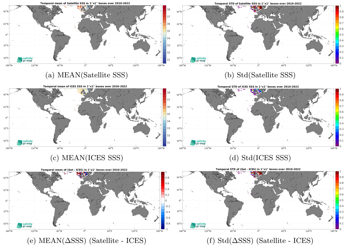
Figure 6: Temporal mean (left) and Std (right) of SSS from SMOS SSS L2Q v331 - 0.25 Deg (CATDS-CPDC) (top), ICES (middle), and of \Delta SSS (Satellite - ICES). Only match-up pairs are used to generate these maps.
