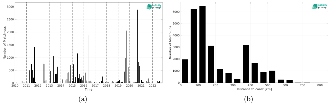
Figure 1: Number of match-ups between ICES and SMOS SSS L2Q v331 - 0.25 Deg (CATDS-CPDC) SSS as a function of time (a) and as function of the distance to coast (b) over the SMOS coastal zone (<800km) 60N-60S Pi-MEP region and for the full satellite product period.
