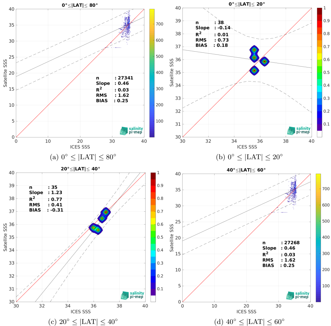
Figure 9: Contour maps of the concentration of SMOS SSS L2Q v331 - 0.25 Deg (CATDS-CPDC) SSS (y-axis) versus ICES SSS (x-axis) at match-up pairs for different latitude bands. For each plot, the red line shows x=y . The black thin and dashed lines indicate a linear fit through the data cloud and the \pm 95\% confidence levels, respectively. The number match-up pairs n , the slope and R^2 coefficient of the linear fit, the root mean square (RMS) and the mean bias between satellite and in situ data are indicated for each latitude band in each plots.
