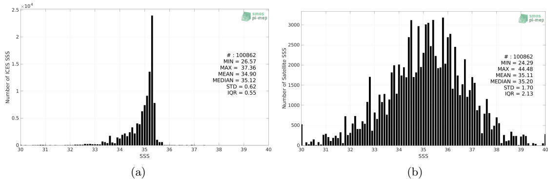
Figure 2: Histograms of SSS from ICES (a) and SMOS SSS L2Q v331 - 0.25 Deg (CATDS-CPDC) (b) considering all match-up pairs per bins of 0.1 over the SMOS coastal zone (<800km) 60N-60S Pi-MEP region and for the full satellite product period.
