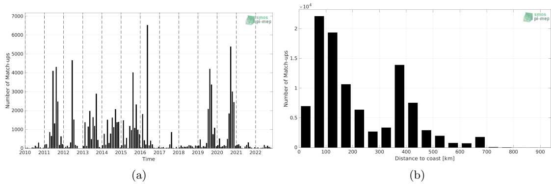
Figure 1: Number of match-ups between ICES and SMOS SSS L2Q v331 - 0.25 Deg (CATDS-CPDC) SSS as a function of time (a) and as function of the distance to coast (b) over the SMOS coastal zone (<800km) 60N-60S Pi-MEP region and for the full satellite product period.
