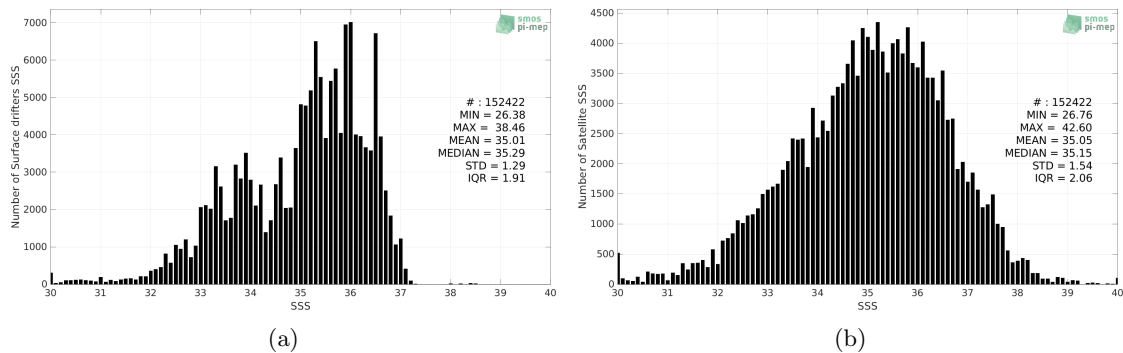
Figure 2: Histograms of SSS from Surface drifters (a) and SMOS SSS L2Q v331 - 0.25 Deg (CATDS-CPDC) (b) considering all match-up pairs per bins of 0.1 over the SMOS coastal zone (<800km) 60N-60S Pi-MEP region and for the full satellite product period.
