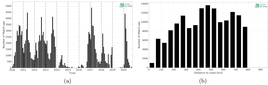
Figure 1: Number of match-ups between Surface drifters and SMOS SSS L2Q v331 - 0.25 Deg (CATDS-CPDC) SSS as a function of time (a) and as function of the distance to coast (b) over the SMOS coastal zone (<800km) 60N-60S Pi-MEP region and for the full satellite product period.
