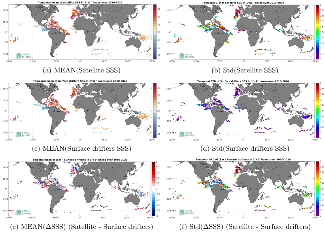
Figure 5: Temporal mean (left) and Std (right) of SSS from SMOS SSS L2Q v331 - 0.25 Deg (CATDS-CPDC) (top), Surface drifters (middle), and of \Delta SSS (Satellite - Surface drifters). Only match-up pairs are used to generate these maps.
