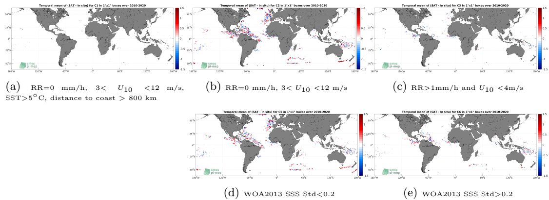
Figure 11: Temporal mean gridded over spatial boxes of size 1^\circ \times 1^\circ of \Delta SSS (SMOS SSS L2Q v331 - 0.25 Deg (CATDS-CPDC) - Surface drifters) for 5 different subdatasets corresponding to:RR=0 mm/h, 3 < U_{10} < 12 m/s, SST >5^\circ C, distance to coast > 800 km (a), RR=0 mm/h, 3 < U_{10} < 12 m/s (b), RR >1 mm/h and U_{10} < 4 m/s (c), WOA2013 SSS Std <0.2 (d), WOA2013 SSS Std >0.2 (e).
