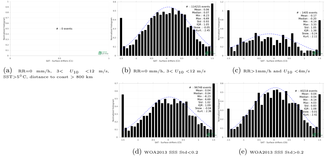
Figure 12: Normalized histogram of \Delta SSS (SMOS SSS L2Q v331 - 0.25 Deg (CATDS-CPDC) - Surface drifters) for 5 different subdatasets corresponding to: RR=0 mm/h, 3 < U_{10} < 12 m/s, SST > 5°C, distance to coast > 800 km (a), RR=0 mm/h, 3 < U_{10} < 12 m/s (b), RR > 1mm/h and U_{10} < 4 m/s (c), WOA2013 SSS Std < 0.2 (d), WOA2013 SSS Std > 0.2 (e).
