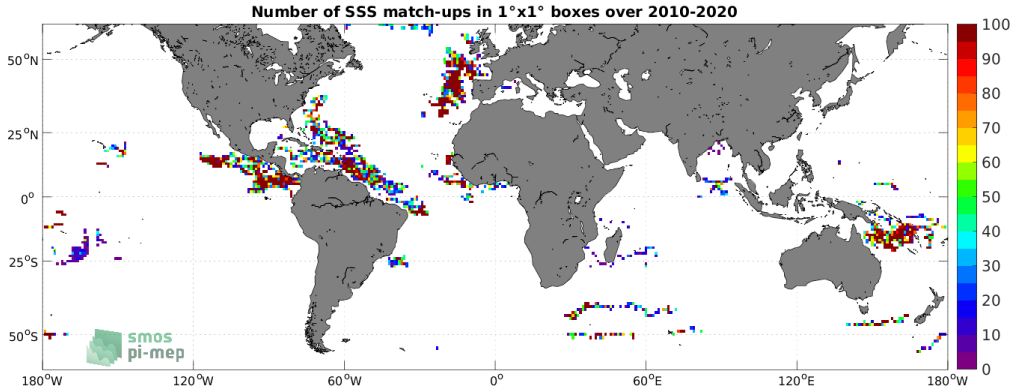
Figure 3: Number of SSS match-ups between Surface drifters SSS and the SMOS SSS L2Q v331 - 0.25 Deg (CATDS-CPDC) SSS product for the SMOS coastal zone (<800km) 60N-60S Pi-MEP region over 1^{\circ} \times 1^{\circ} boxes and for the full satellite product period.
