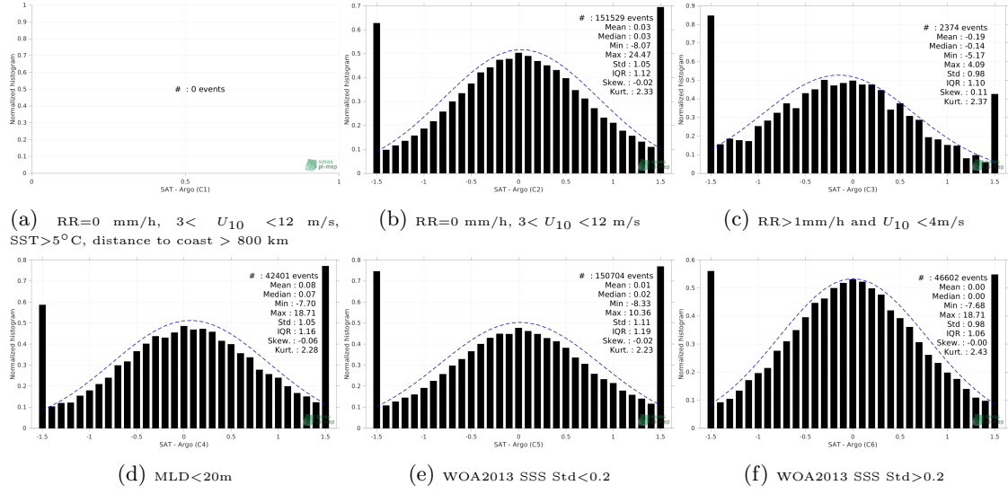
Figure 13: Normalized histogram of \Delta\text{SSS} (SMOS SSS L2Q v331 - 0.25 Deg (CATDS-CPDC) - Argo) for 6 different subdatasets corresponding to: RR=0 mm/h, 3 < U_{10} < 12 m/s, SST>5°C, distance to coast > 800 km (a), RR=0 mm/h, 3 < U_{10} < 12 m/s (b), RR>1mm/h and U_{10} < 4 m/s (c), MLD<20m (d), WOA2013 SSS Std<0.2 (e), WOA2013 SSS Std>0.2 (f).
