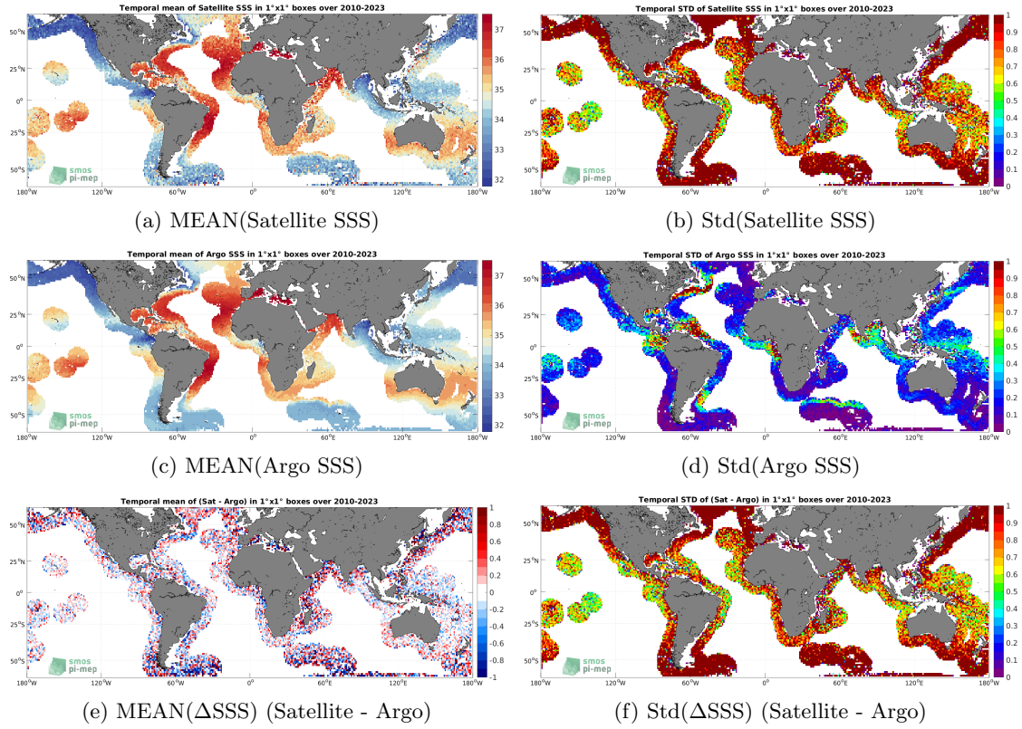
Figure 6: Temporal mean (left) and Std (right) of SSS from SMOS SSS L2Q v331 - 0.25 Deg (CATDS-CPDC) (top), Argo (middle), and of \Delta SSS (Satellite - Argo). Only match-up pairs are used to generate these maps.
