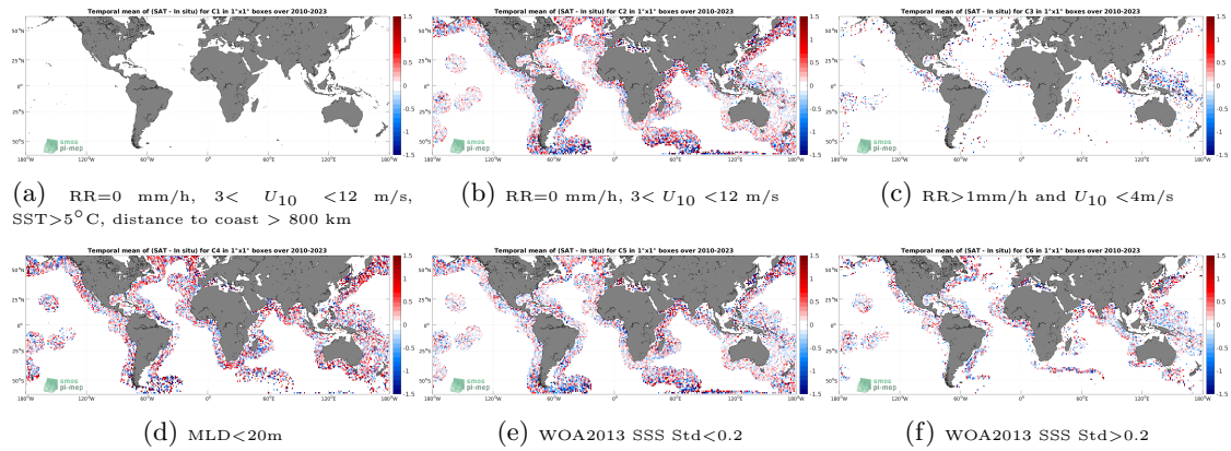
Figure 12: Temporal mean gridded over spatial boxes of size 1^\circ \times 1^\circ of \Delta SSS (SMOS SSS L2Q v331 - 0.25 Deg (CATDS-CPDC) - Argo) for 6 different subdatasets corresponding to:RR=0 mm/h, 3 < U_{10} < 12 m/s, SST >5^\circ C, distance to coast > 800 km (a), RR=0 mm/h, 3 < U_{10} < 12 m/s (b), RR >1 mm/h and U_{10} < 4 m/s (c),MLD <20 m (d),WOA2013 SSS Std <0.2 (e),WOA2013 SSS Std >0.2 (f).
