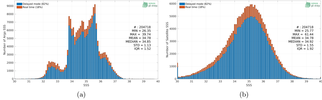
Figure 2: Histograms of SSS from Argo (a) and SMOS SSS L2Q v331 - 0.25 Deg (CATDS-CPDC) (b) considering all match-up pairs per bins of 0.1 over the SMOS coastal zone (<800km) 60N-60S Pi-MEP region and for the full satellite product period.
