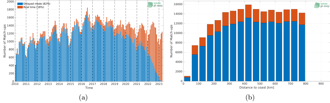
Figure 1: Number of match-ups between Argo and SMOS SSS L2Q v331 - 0.25 Deg (CATDS-CPDC) SSS as a function of time (a) and as function of the distance to coast (b) over the SMOS coastal zone (<800km) 60N-60S Pi-MEP region and for the full satellite product period.
