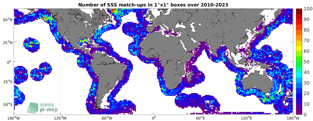
Figure 4: Number of SSS match-ups between Argo SSS and the SMOS SSS L2Q v331 - 0.25 Deg (CATDS-CPDC) SSS product for the SMOS coastal zone (<800km) 60N-60S Pi-MEP region over 1^\circ \times 1^\circ boxes and for the full satellite product period.
