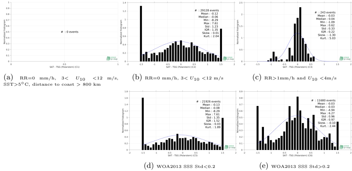
Figure 13: Normalized histogram of \Delta SSS (SMOS SSS L2Q v330 - 0.25 Deg (CATDS-CPDC) - TSG (Polarstern)) for 5 different subdatasets corresponding to: RR=0 mm/h, 3 < U_{10} < 12 m/s, SST>5°C, distance to coast > 800 km (a), RR=0 mm/h, 3 < U_{10} < 12 m/s (b), RR>1mm/h and U_{10} < 4 m/s (c), WOA2013 SSS Std<0.2 (d), WOA2013 SSS Std>0.2 (e).
