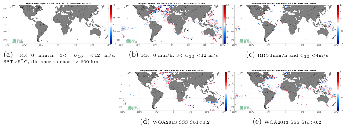
Figure 12: Temporal mean gridded over spatial boxes of size 1^\circ \times 1^\circ of \Delta\text{SSS} (SMOS SSS L2Q v330 - 0.25 Deg (CATDS-CPDC) - TSG (LEGOS-DM)) for 5 different subdatasets corresponding to:RR=0 mm/h, 3 < U_{10} < 12 m/s, SST >5^\circ\text{C} , distance to coast > 800 km (a), RR=0 mm/h, 3 < U_{10} < 12 m/s (b), RR >1 mm/h and U_{10} < 4 m/s (c), WOA2013 SSS Std <0.2 (d), WOA2013 SSS Std >0.2 (e).
