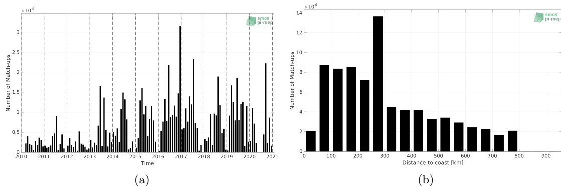
Figure 1: Number of match-ups between TSG (GOSUD-Research-vessel) and SMOS SSS L2Q v330 - 0.25 Deg (CATDS-CPDC) SSS as a function of time (a) and as function of the distance to coast (b) over the SMOS coastal zone (<800km) 60N-60S Pi-MEP region and for the full satellite product period.
