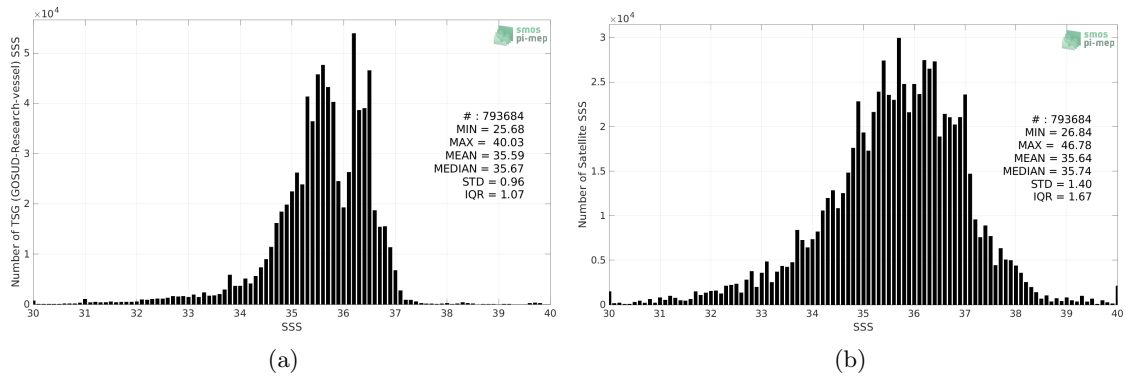
Figure 2: Histograms of SSS from TSG (GOSUD-Research-vessel) (a) and SMOS SSS L2Q v330 - 0.25 Deg (CATDS-CPDC) (b) considering all match-up pairs per bins of 0.1 over the SMOS coastal zone (<800km) 60N-60S Pi-MEP region and for the full satellite product period.
