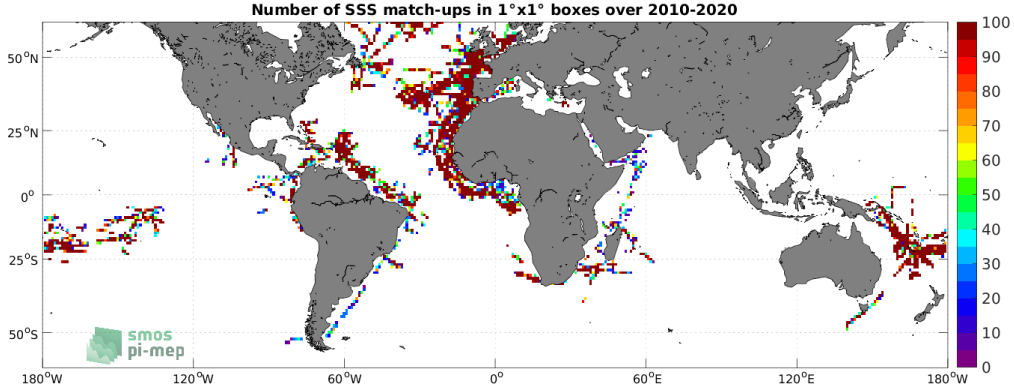
Figure 4: Number of SSS match-ups between TSG (GOSUD-Research-vessel) SSS and the SMOS SSS L2Q v330 - 0.25 Deg (CATDS-CPDC) SSS product for the SMOS coastal zone (<800km) 60N-60S Pi-MEP region over 1^\circ \times 1^\circ boxes and for the full satellite product period.
