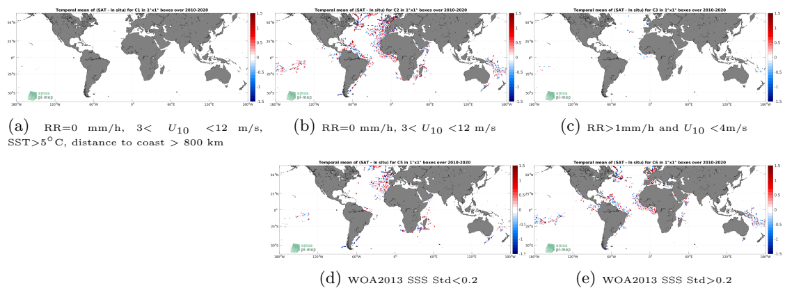
Figure 12: Temporal mean gridded over spatial boxes of size 1^\circ \times 1^\circ of \Delta\text{SSS} (SMOS SSS L2Q v330 - 0.25 Deg (CATDS-CPDC) - TSG (GOSUD-Research-vessel)) for 5 different subdatasets corresponding to:RR=0 mm/h, 3 < U_{10} < 12 m/s, SST >5^\circ\text{C} , distance to coast > 800 km (a), RR=0 mm/h, 3 < U_{10} < 12 m/s (b), RR >1 mm/h and U_{10} < 4 m/s (c), WOA2013 SSS Std <0.2 (d), WOA2013 SSS Std >0.2 (e).
