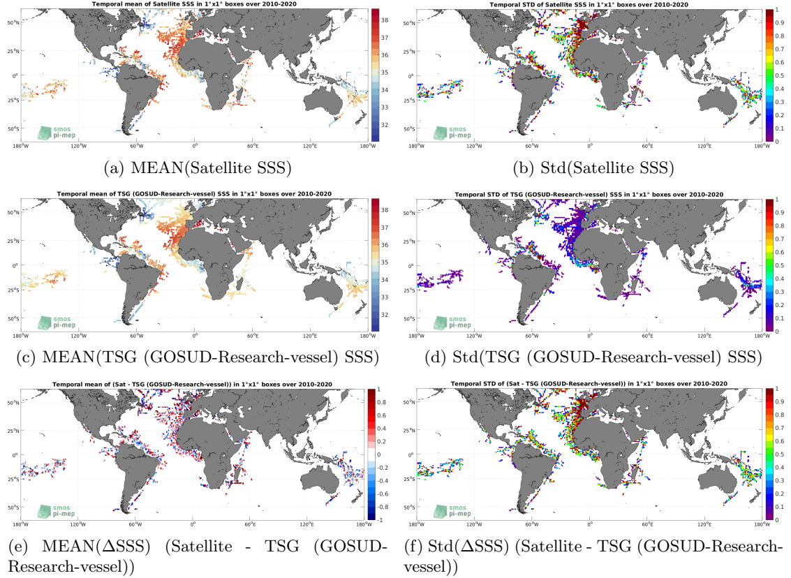
Figure 6: Temporal mean (left) and Std (right) of SSS from SMOS SSS L2Q v330 - 0.25 Deg (CATDS-CPDC) (top), TSG (GOSUD-Research-vessel) (middle), and of \Delta SSS (Satellite - TSG (GOSUD-Research-vessel)). Only match-up pairs are used to generate these maps.
