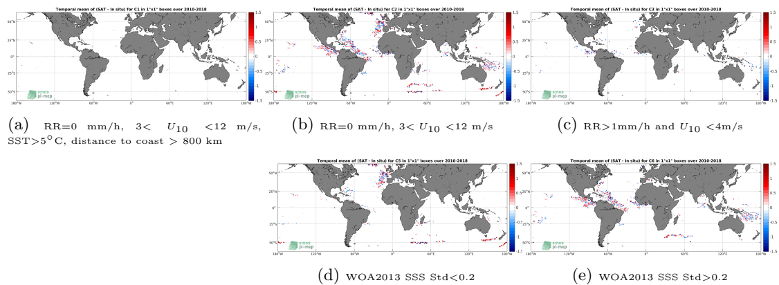
Figure 11: Temporal mean gridded over spatial boxes of size 1^\circ \times 1^\circ of \Delta\text{SSS} (SMOS SSS L2Q v330 - 0.25 Deg (CATDS-CPDC) - Surface drifters) for 5 different subdatasets corresponding to: RR=0 mm/h, 3 < U_{10} < 12 m/s, SST > 5^\circ\text{C} , distance to coast > 800 km (a), RR=0 mm/h, 3 < U_{10} < 12 m/s (b), RR > 1 mm/h and U_{10} < 4 m/s (c), WOA2013 SSS Std < 0.2 (d), WOA2013 SSS Std > 0.2 (e).
